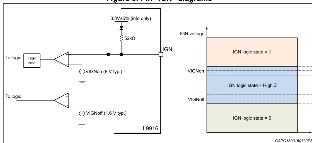
Figure 8. Pin "IGN" diagrams
