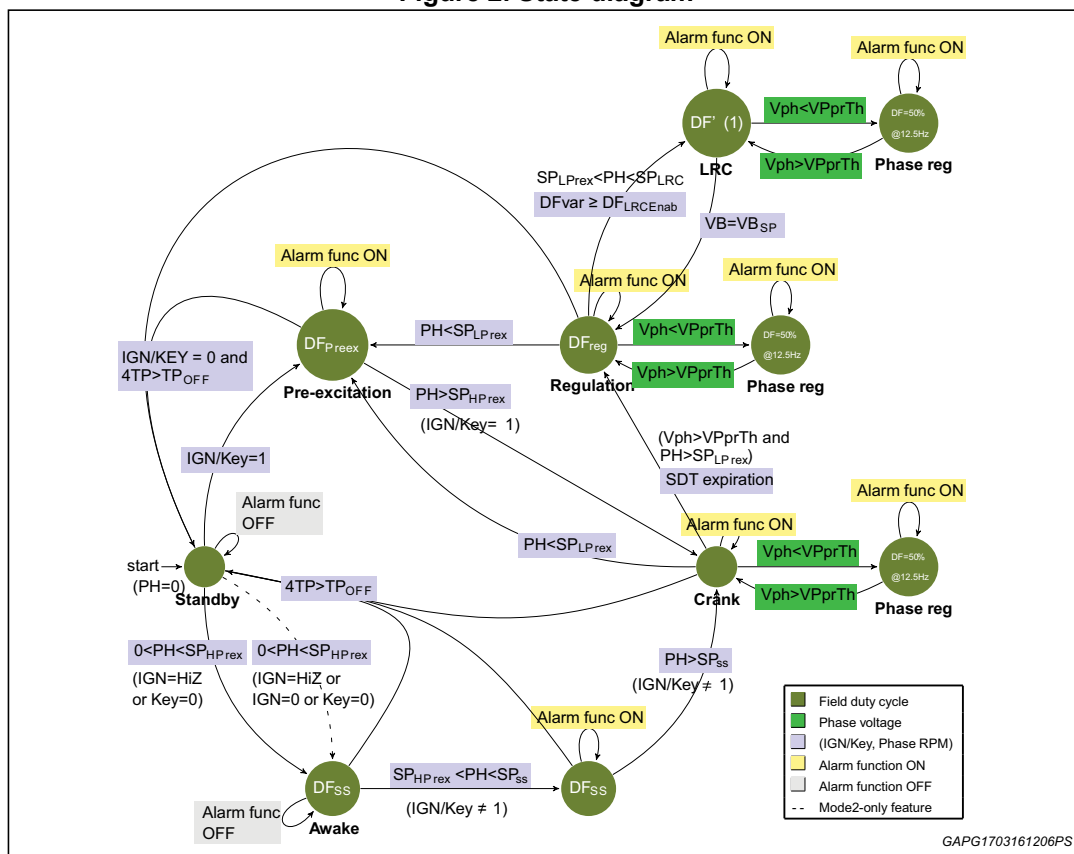
Figure 2. State diagram
