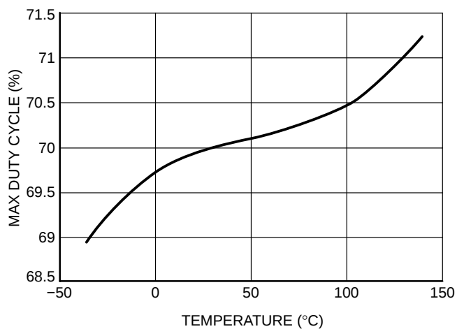
Figure 10. Max Duty Cycle vs. Temperature
