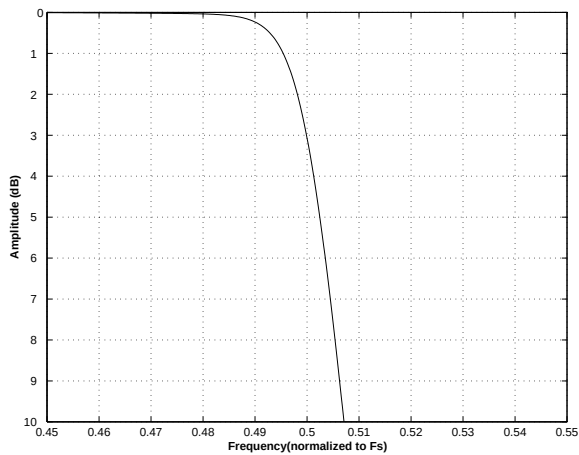
Figure 41. Single-Speed (fast) Transition Band (detail)
