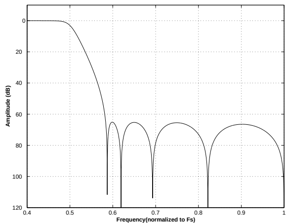
Figure 43. Single-Speed (slow) Stopband Rejection
