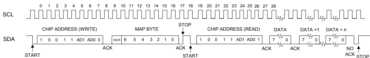
Figure 23. Control Port Timing, I²C Read
