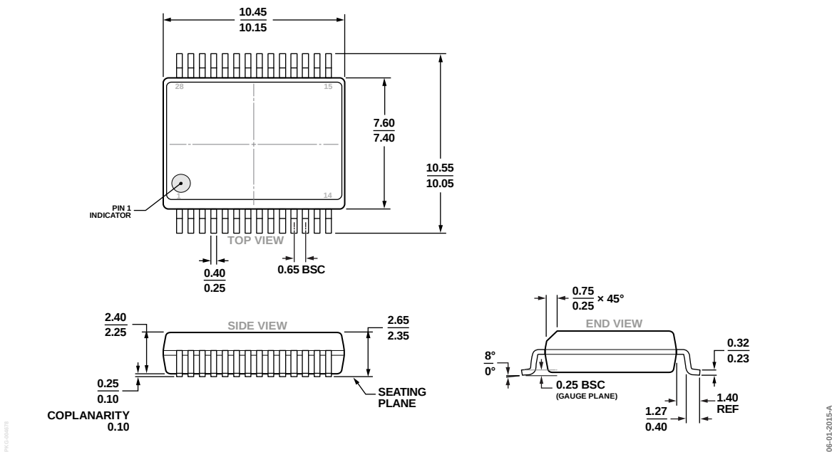
Figure 57. 28-Lead Standard Small Outline, Wide Body, with Finer Pitch [SOIC_W_FP] (RN-28-1)
