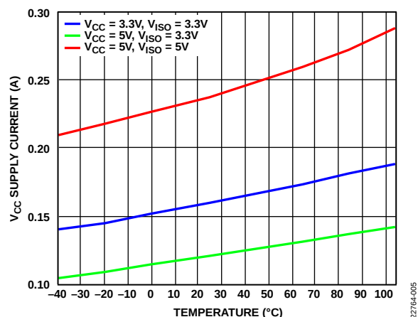
Figure 19. V CC Supply Current vs. Temperature at 25 Mbps, 120 Ω Load, 25 Mbps Models (ADM2565E and ADM2567E)
