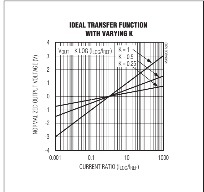
Figure 3. Ideal Transfer Function with Varying K
