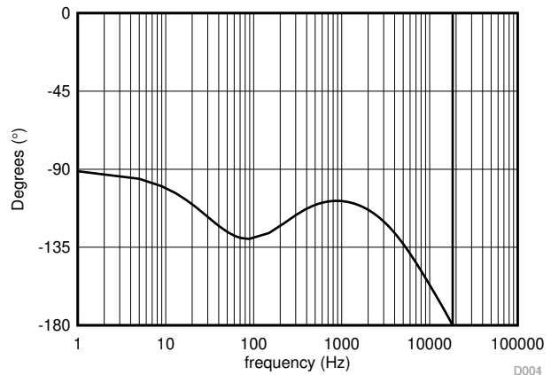
Figure 9-7. Converter Closed-Loop Bode Plot – Phase
