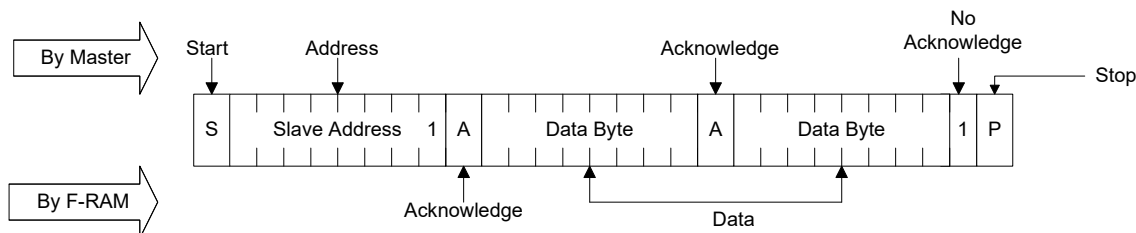
Figure 20. Sequential Read
