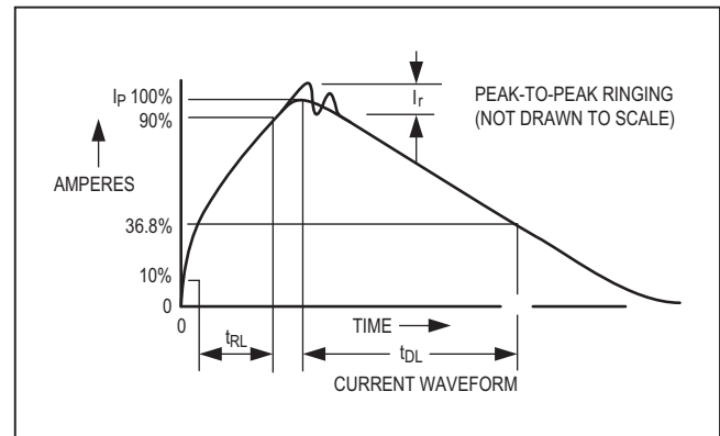
Figure 8. Human Body Current Waveform
