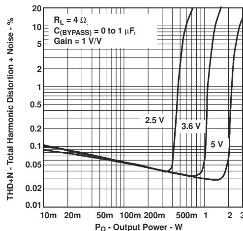
Figure 6-6. Total Harmonic Distortion + Noise vs Output Power
