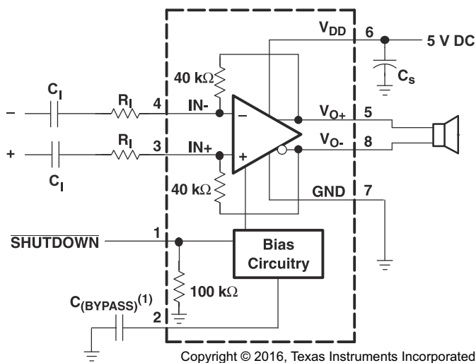
Figure 8-6. Differential Input Application Schematic Optimized With Input Capacitors
