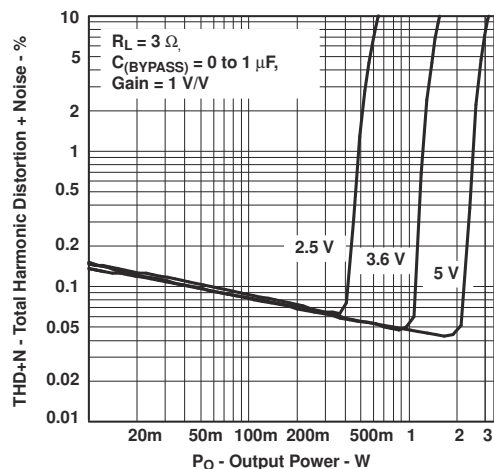
Figure 6-5. Total Harmonic Distortion + Noise vs Output Power
