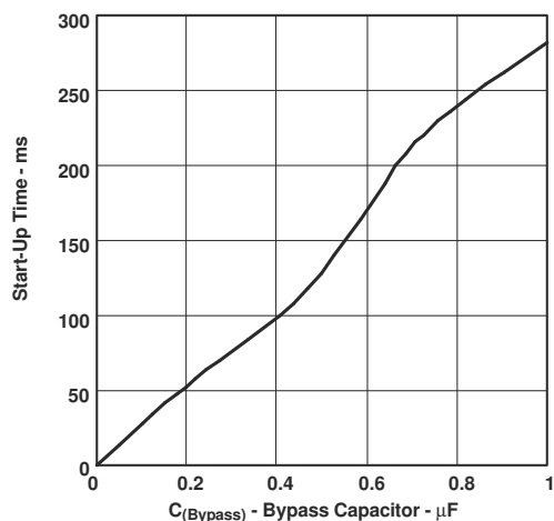
Figure 6-27. Start-up Time vs Bypass Capacitor
