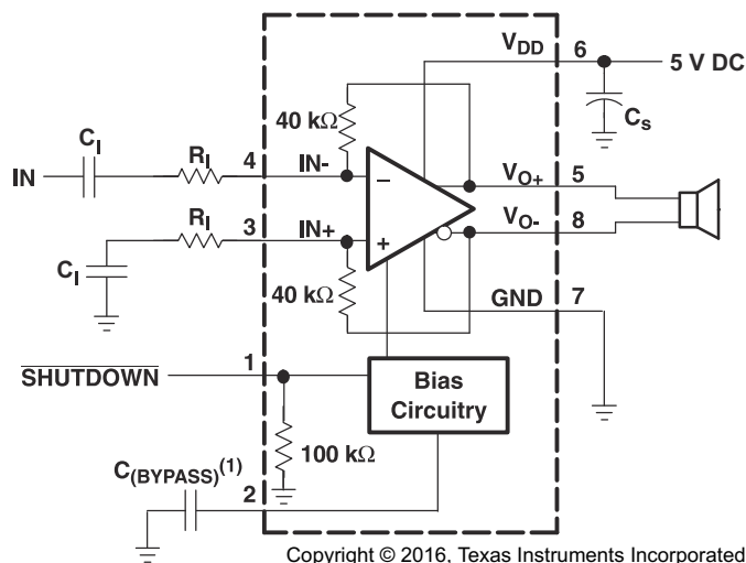
Figure 8-7. Single-Ended Input Application Schematic
