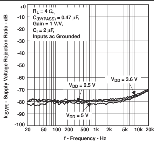
Figure 6-14. Supply Voltage Rejection Ratio vs Frequency
