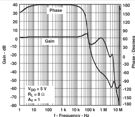
Figure 6-23. Closed Loop Gain/Phase vs Frequency
