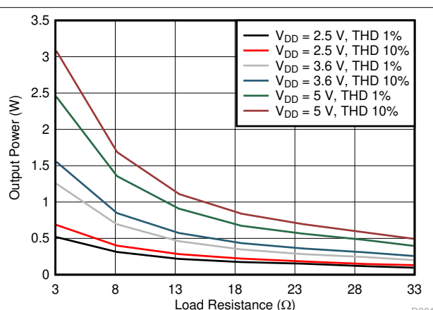
Figure 8-5. Output Power vs Load Resistance
