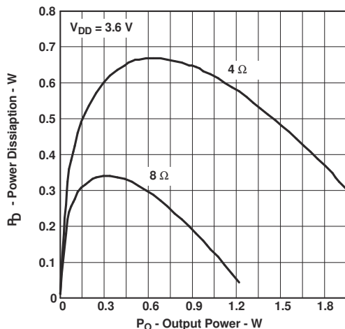
Figure 6-3. Power Dissipation vs Output Power
