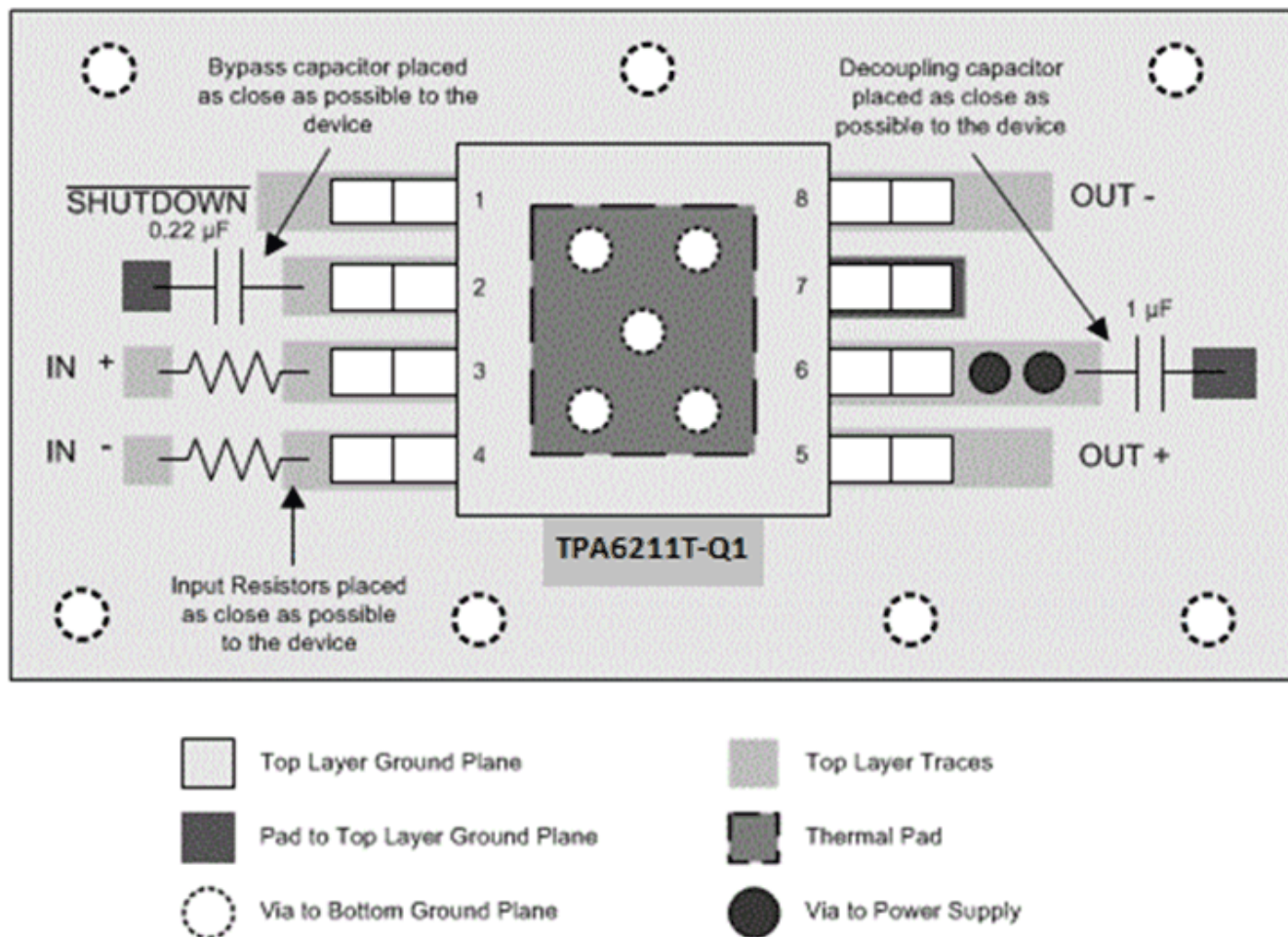
Figure 10-1. TPA6211T-Q1 8-Pin HVSSOP (DGN) Board Layout
