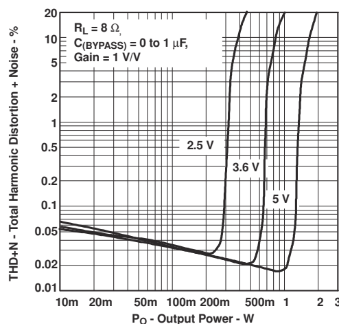
Figure 6-7. Total Harmonic Distortion + Noise vs Output Power
