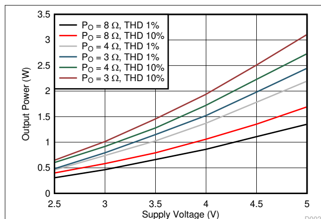
Figure 8-4. Output Power vs Supply Voltage
