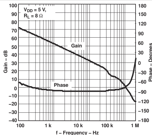
Figure 6-24. Open Loop Gain/Phase vs Frequency
