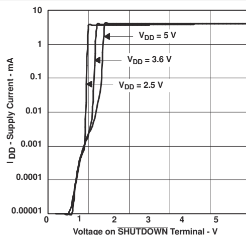
Figure 6-26. Supply Current vs Shutdown Voltage
