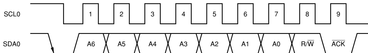
Figure 19-11. Acknowledge Signal
