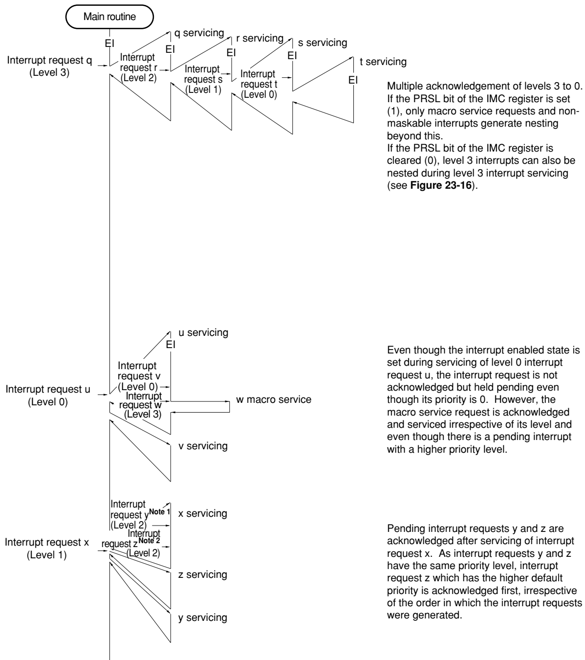
Figure 23-14. Examples of Servicing When Another Interrupt Request Is Generated During Interrupt Service (3/3)
