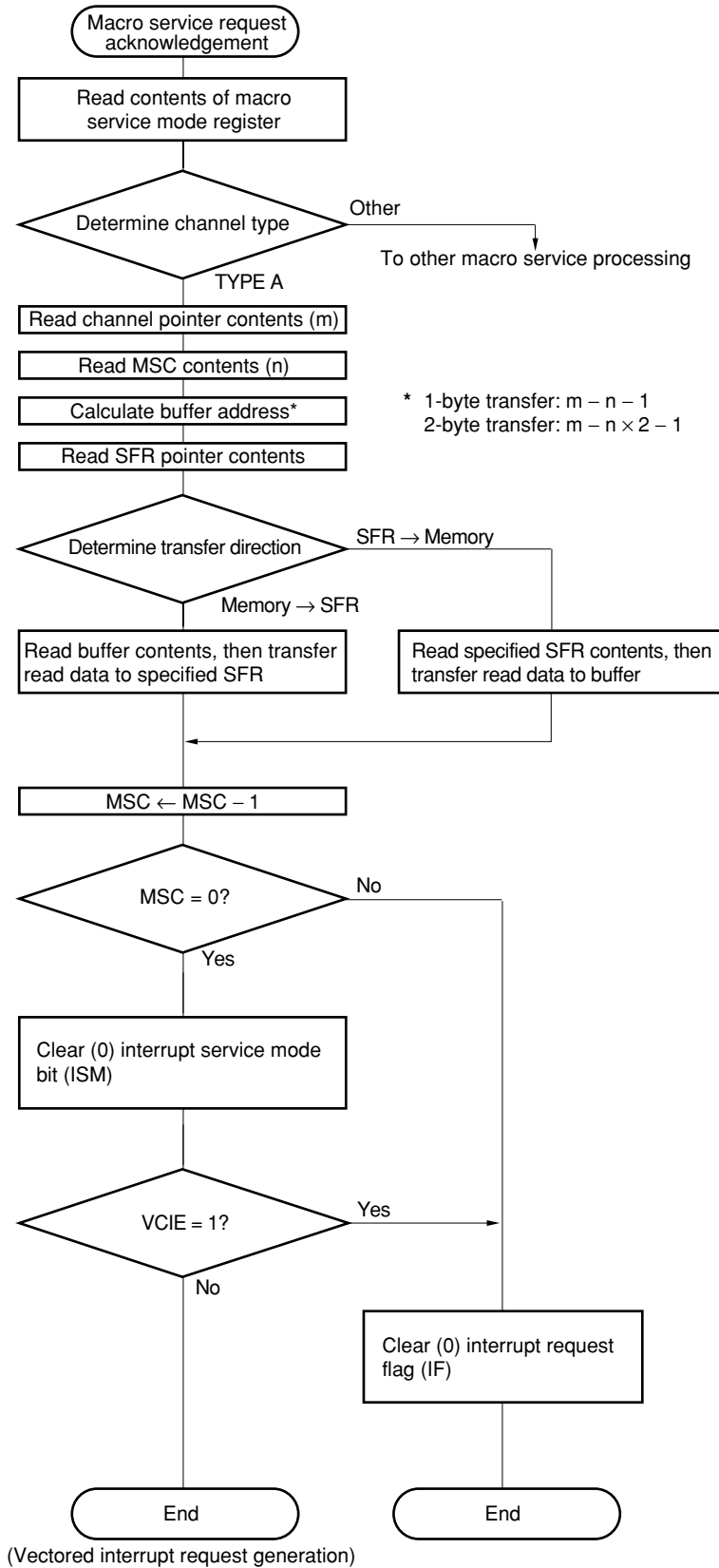
Figure 23-23. Macro Service Data Transfer Processing Flow (Type A)
