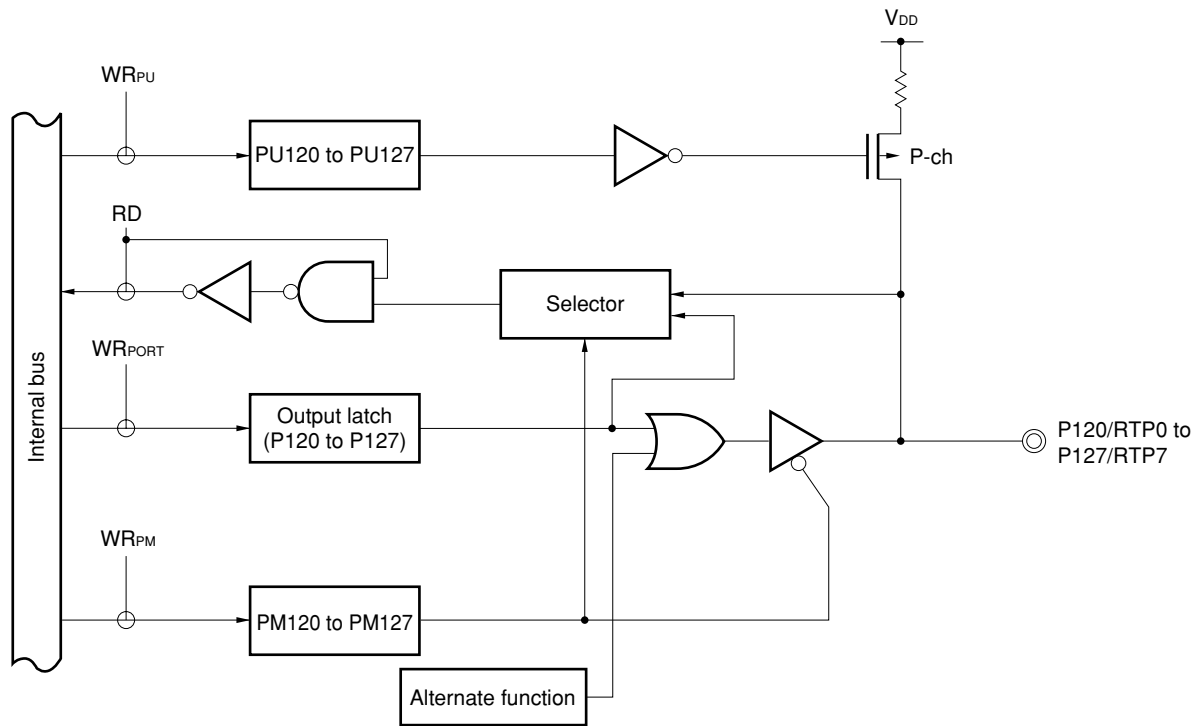
Figure 5-22. Block Diagram of P120 to P127
