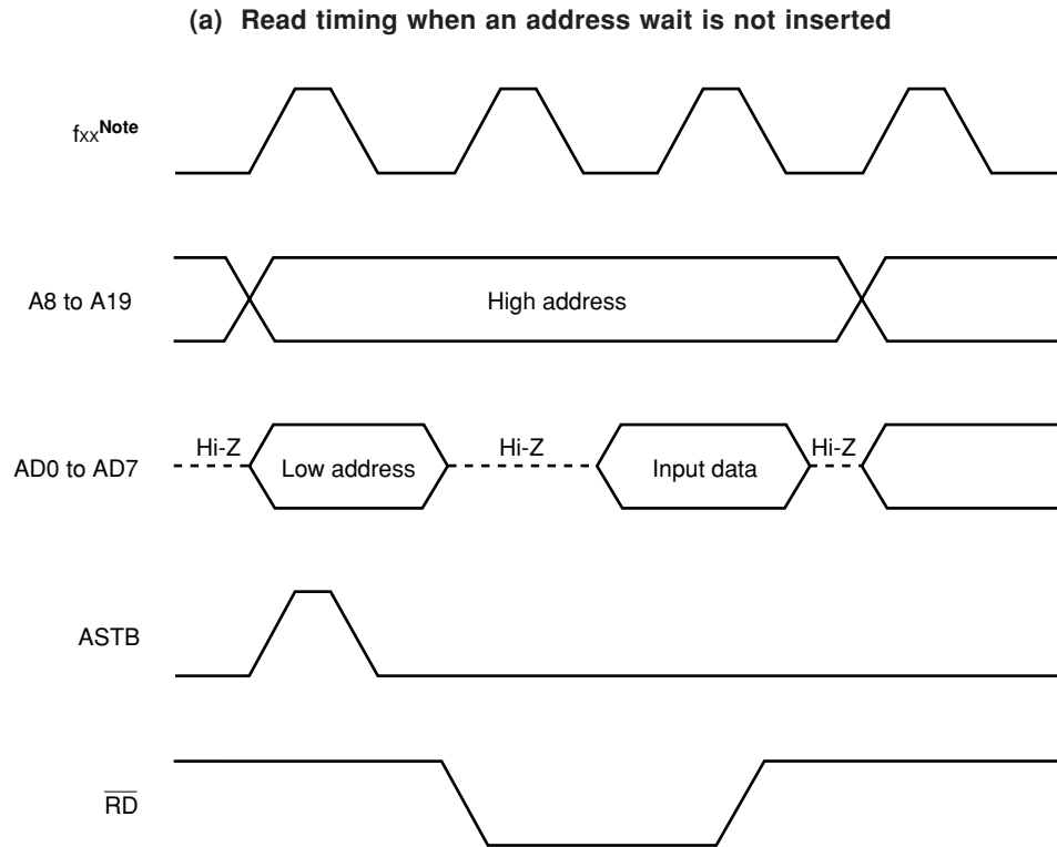
Figure 24-17. Read/Write Timing by Address Wait Function (1/3)
