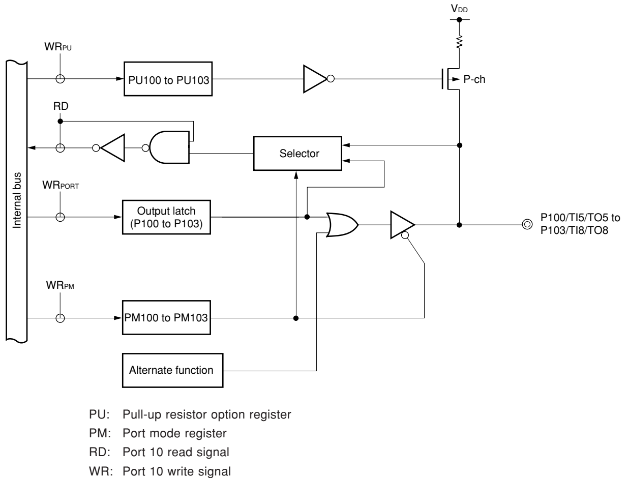
Figure 5-21. Block Diagram of P100 to P103
