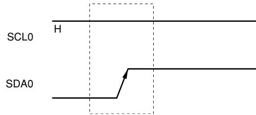
Figure 19-12. Stop Condition
