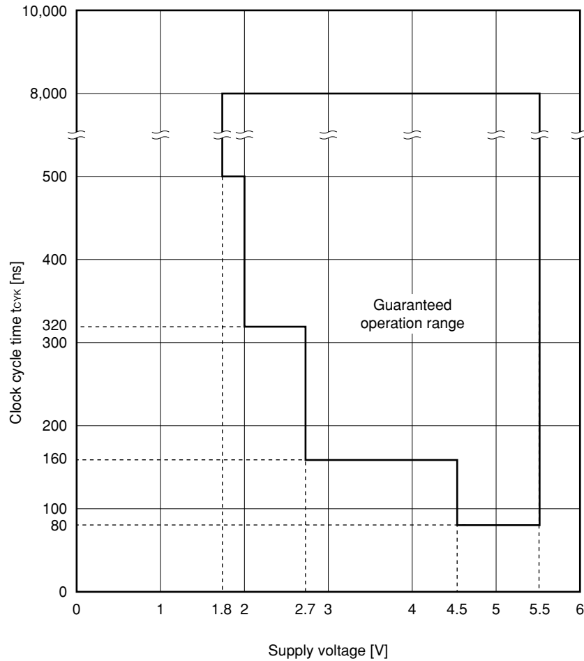
Figure 30-1. Power Supply Voltage and Clock Cycle Time (CPU Clock Frequency: f_{CPU} )
