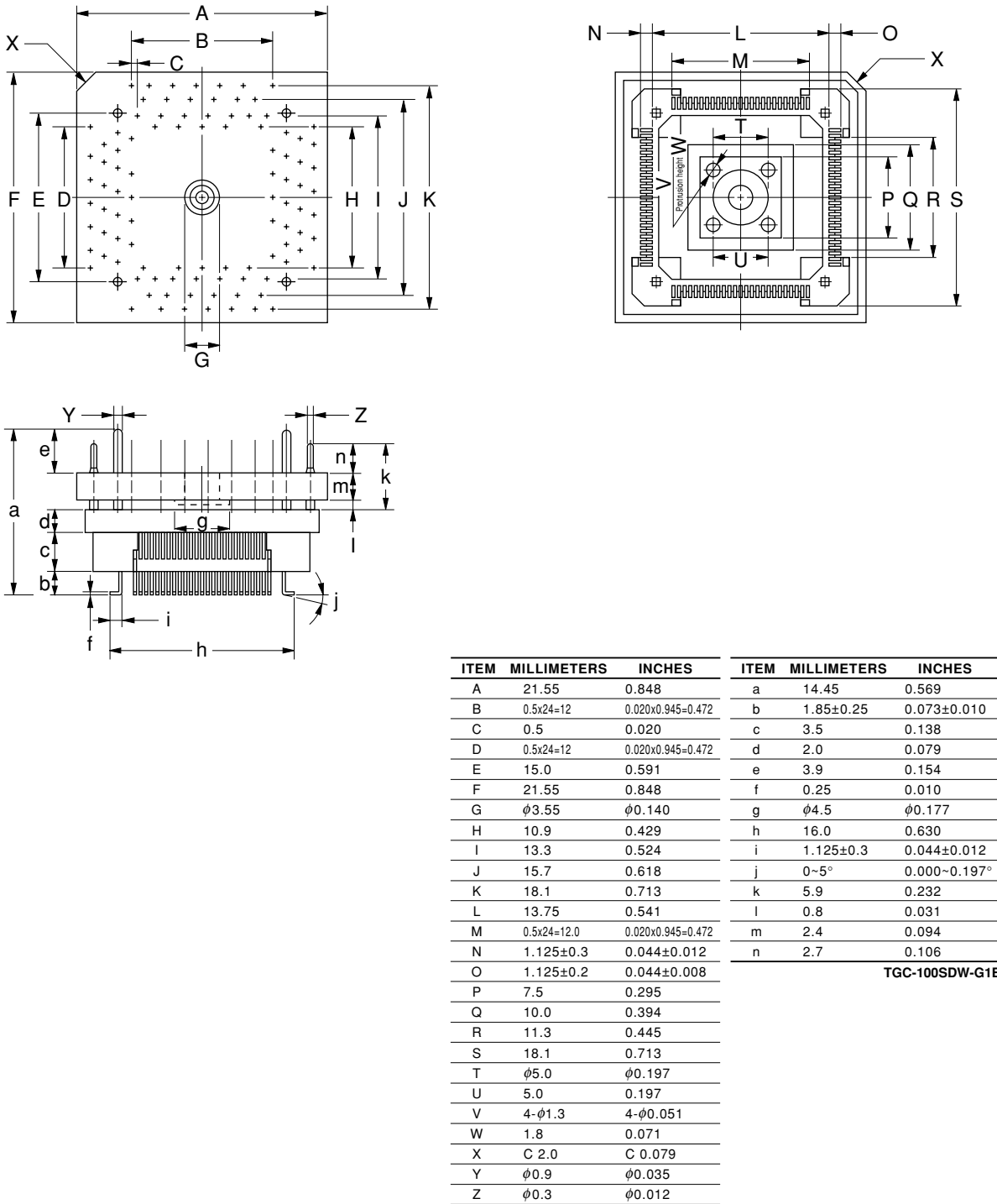
Figure B-9. Package Drawing of TGC-100SDW (Reference)
