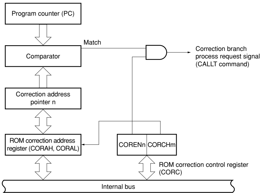
Figure 27-1. ROM Correction Block Diagram
