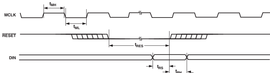
Figure 1. MCLK and \overline{\text{RESET}} Timing
