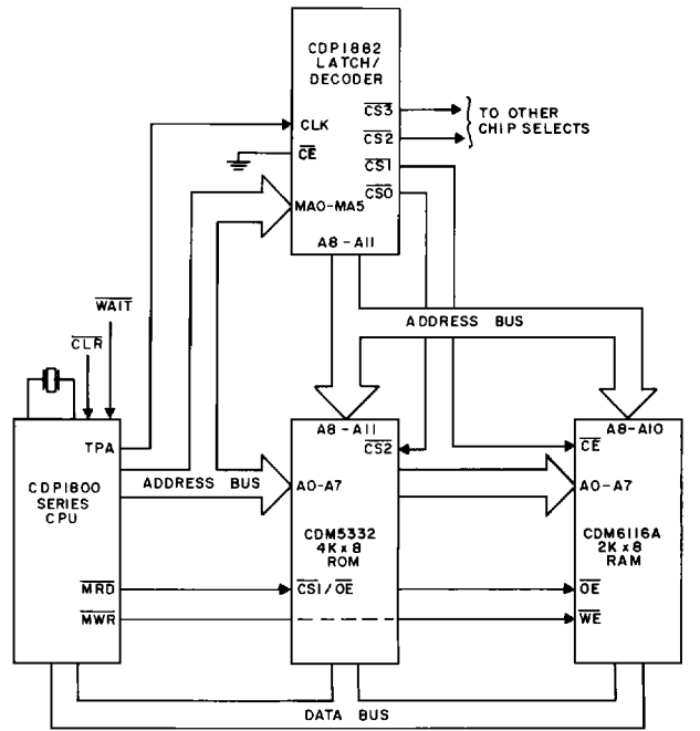
Fig. 5 - CDP1800-series system using the CDP1882.
