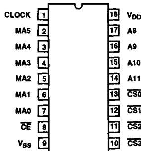
CDP1882, CDP1882C 18 LEAD DIP TOP VIEW
