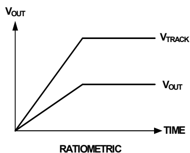
FIGURE 9. TRACKING MODES
