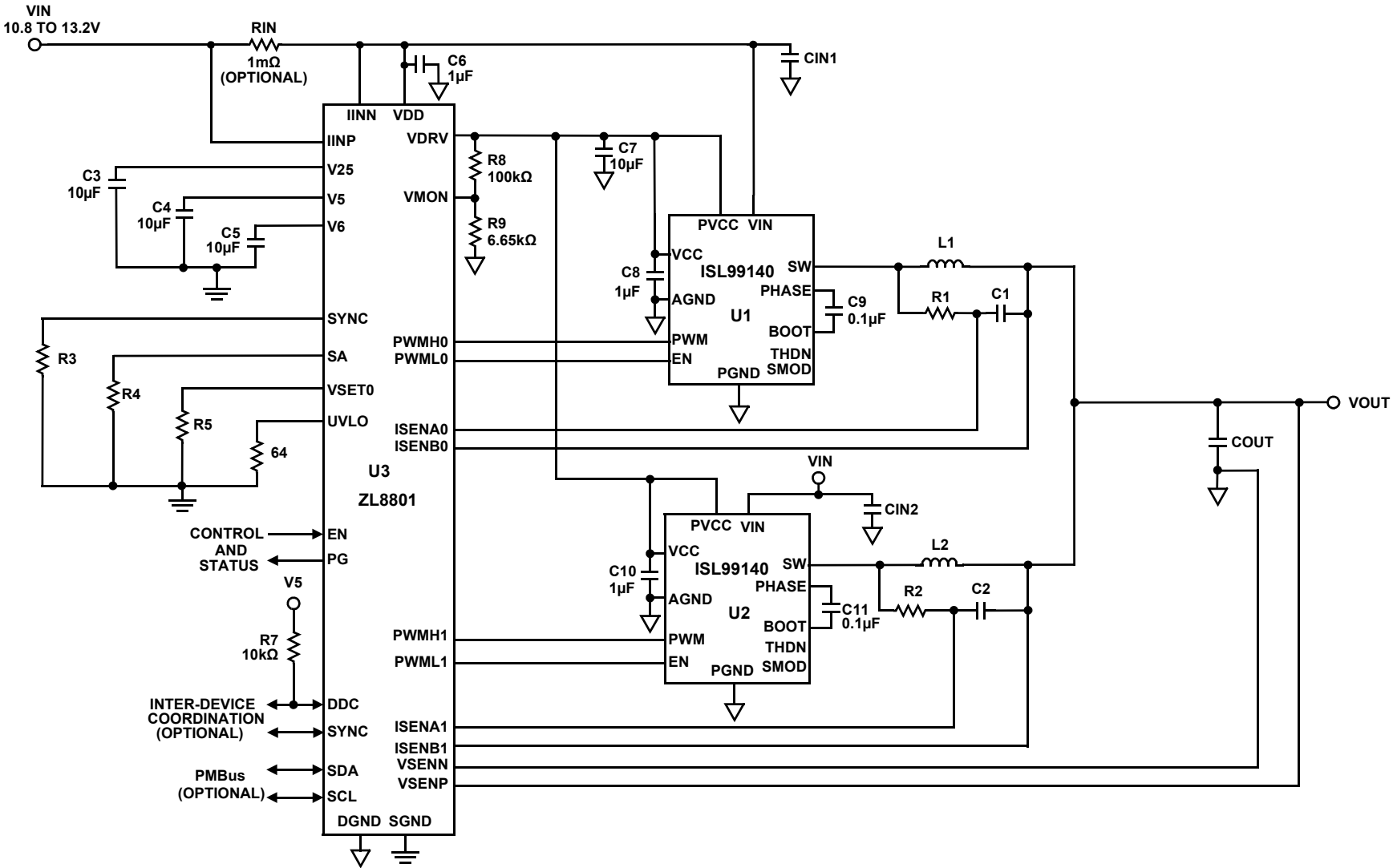
FIGURE 3. ZL8801 SCHEMATIC
