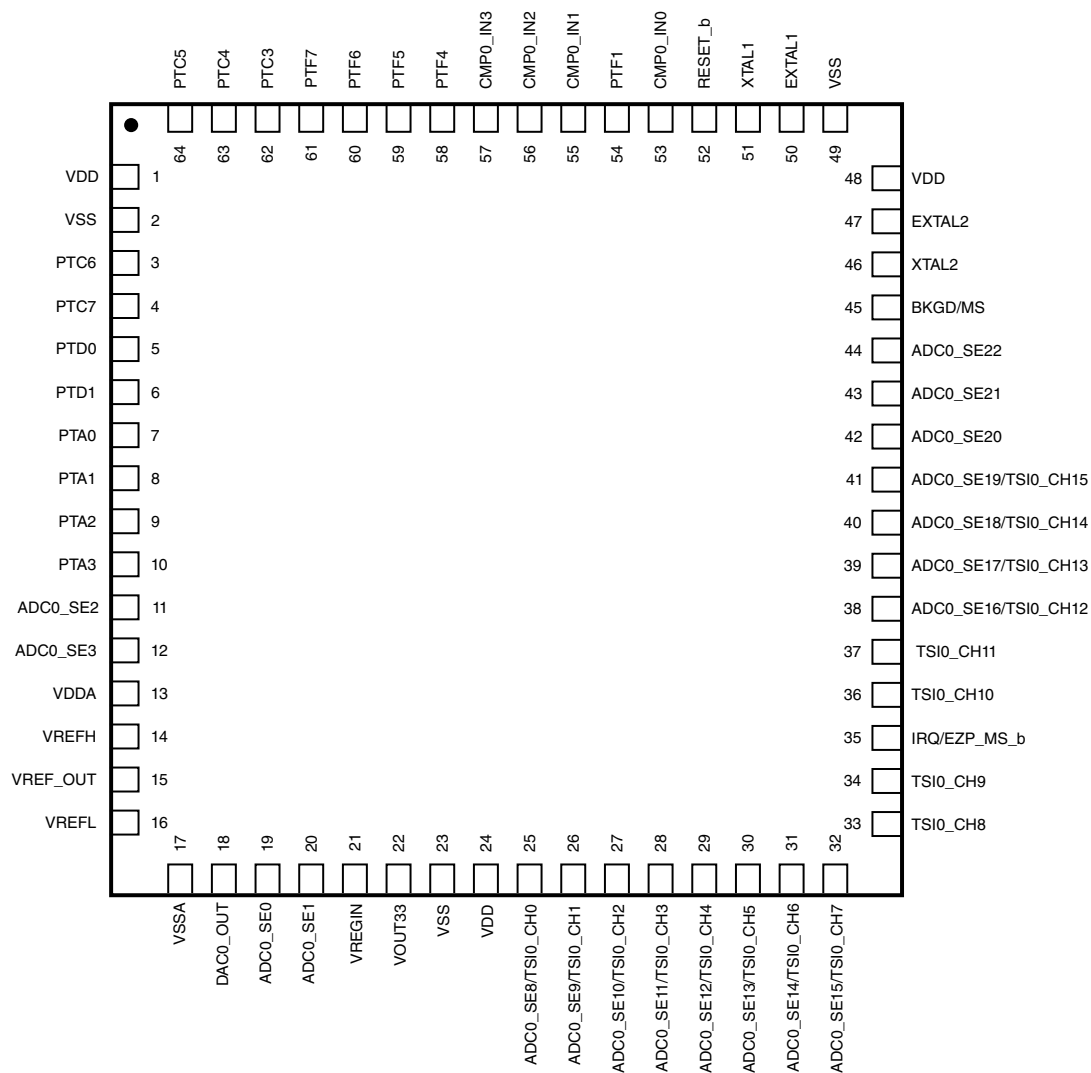
Figure 18. 64-pin LQFP
