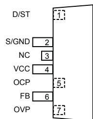
Pin-out Diagrams
