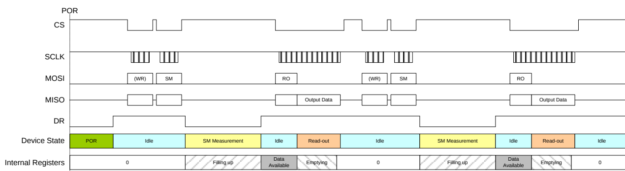
Figure 19: Global timing diagram with separate SM-RO
