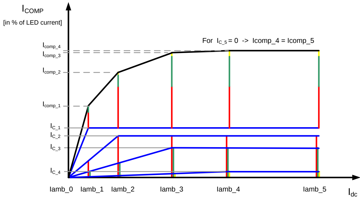
Figure 4: Example of a compensation curve I_{COMP} for I_{C5}=0 . The dc-currents of the corner points are fixed in the design and cannot be influenced. The compensation components I_{C1}...I_{C5} are defined by the registers DC_COMP_IC1...5 with 4 bits each. The resulting compensation characteristics are shown in the black graph.
