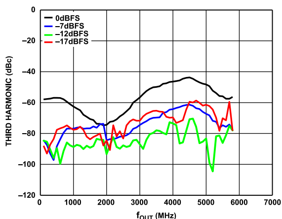
Figure 16. Third Harmonic (dBc) vs. f_{OUT} over Digital Scale (Mode 9), 12 GHz DAC Sample Rate, Channel Interpolation 1 \times , Main Interpolation 12 \times
