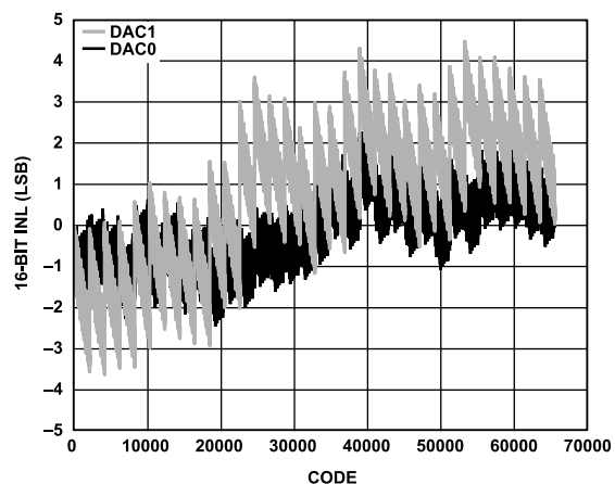
Figure 34. INL, I_{OUTFS} = 26 mA, 16-Bit Resolution
