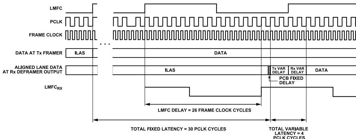
Figure 62. LMFC Delay Calculation Example
