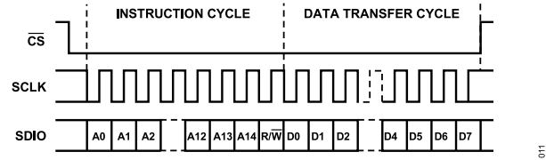
Figure 45. Serial Register Interface Timing, LSB First, Register 0x000, Bit 6 and Bit 1 = 1
