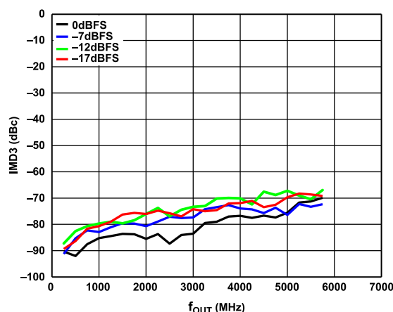
Figure 19. IMD3 vs. f_{OUT} over Digital Scale (Mode 1), 12 GHz DAC Sample Rate, Channel Interpolation 4 \times , Main Interpolation 8 \times , 1 MHz Tone Spacing
