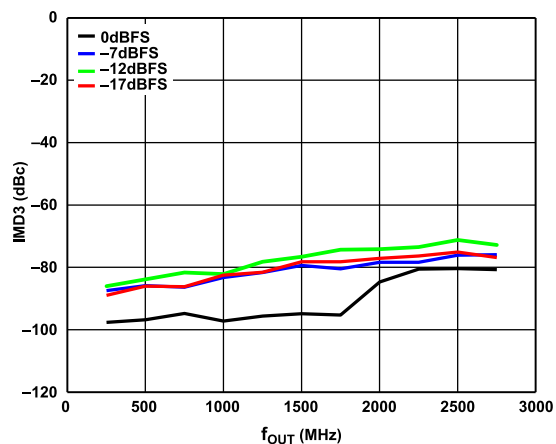
Figure 17. IMD3 vs. f_{OUT} over Digital Scale (Mode 0) 6 GHz DAC Sample Rate, Channel Interpolation 2 \times , Main Interpolation 8 \times , 1 MHz Tone Spacing
