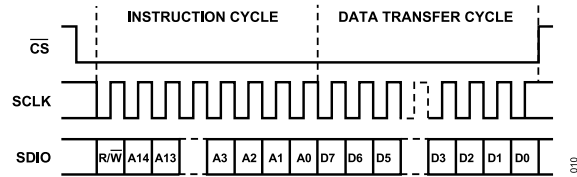
Figure 44. Serial Register Interface Timing, MSB First, Register 0x000, Bit 6 and Bit 1 = 0
