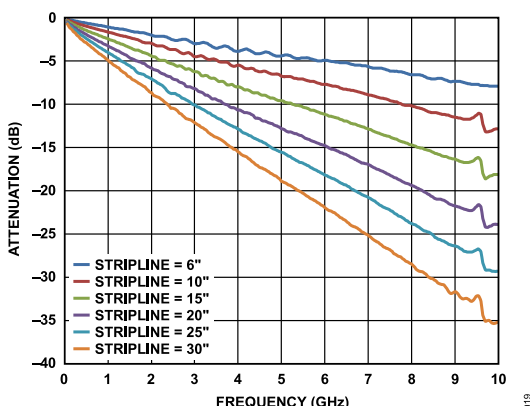
Figure 53. Insertion Loss of 50 \Omega Striplines on FR4
