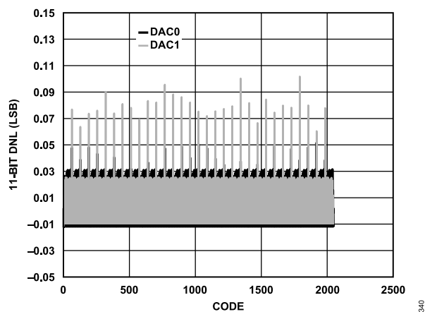
Figure 41. DNL, I_{OUTFS} = 20\text{ mA} , 11-Bit Resolution
