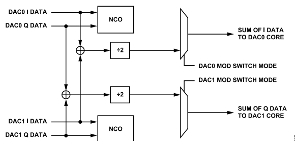
Figure 78. Mode 1—DAC0 = I0 + I1, DAC1 = Q0 + Q1
