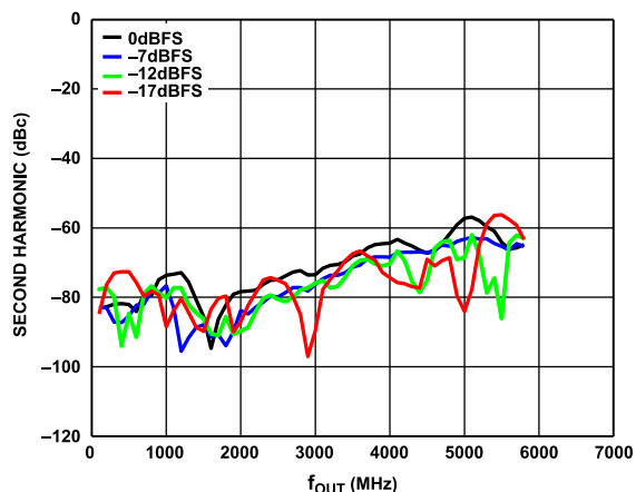
Figure 15. Second Harmonic (dBc) vs. f_{OUT} over Digital Scale (Mode 9), 12 GHz DAC Sample Rate, Channel Interpolation 1 \times , Main Interpolation 12 \times
