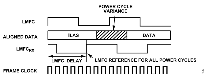
Figure 61. LMFC_DELAY_x to Compensate for Link Delay &gt; LMFC
