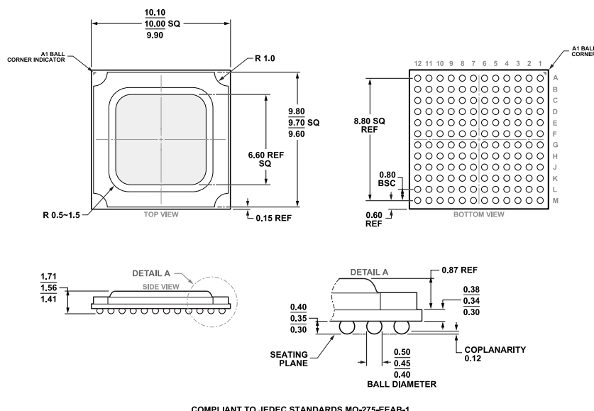
Figure 90. 144-Ball Ball Grid Array, Thermally Enhanced [BGA_ED] (BP-144-1) Dimensions shown in millimeters
