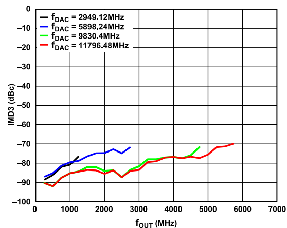
Figure 20. IMD3 vs. f_{OUT} over f_{DAC} (Mode 1), Channel Interpolation 4 \times , Main Interpolation 8 \times , 1 MHz Tone Spacing, -7 dB Digital Scale
