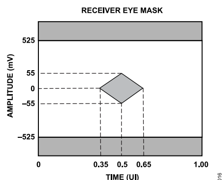
Figure 50. Receiver Eye Mask
