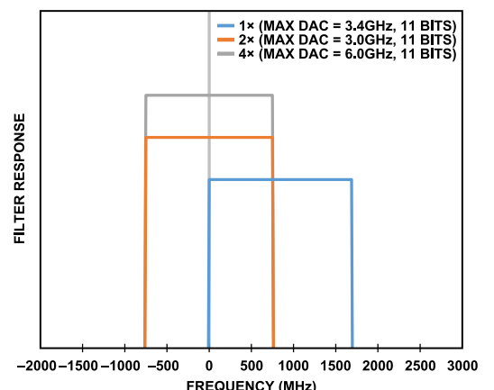
Figure 66. Band Responses of Total Interpolation Rates for 1×, 2×, and 4× at Each Respective Maximum Achievable DAC Rate, 11-Bit Resolution
