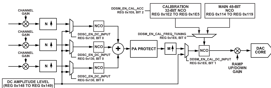
Figure 68. DC Amplitude Injection for NCO Only Mode Block Diagram
