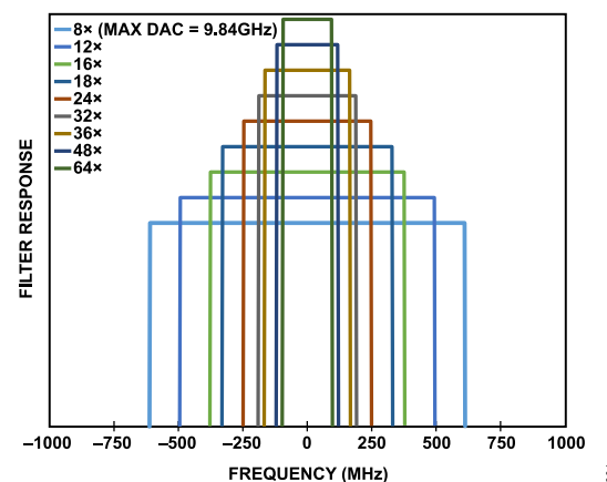
Figure 67. Band Responses of Total Interpolation Rates for 8×, 12×, 16×, 18×, 24×, 32×, 36×, 48×, and 64× at a 12 GHz DAC Rate, 16-Bit Resolution (Unless Otherwise Noted)
