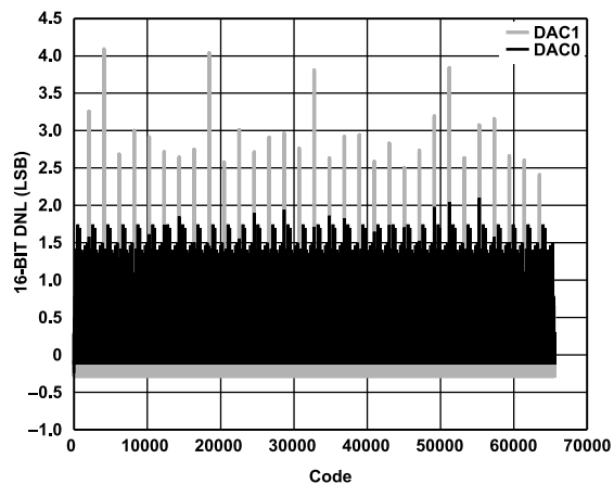
Figure 35. DNL, I_{OUTFS} = 20 mA, 16-Bit Resolution
