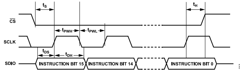
Figure 47. Timing Diagram for Serial Port Register Write
