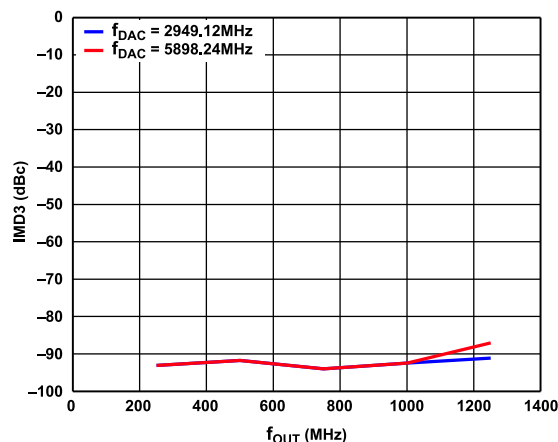
Figure 18. IMD3 vs. f_{OUT} over f_{DAC} (Mode 0), Channel Interpolation 2 \times , Main Interpolation 8 \times , 1 MHz Tone Spacing
