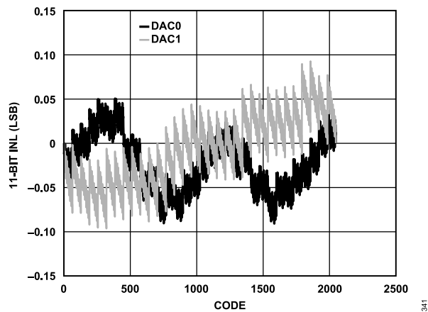
Figure 42. INL, I_{OUTFS} = 20\text{ mA} , 11-Bit Resolution
