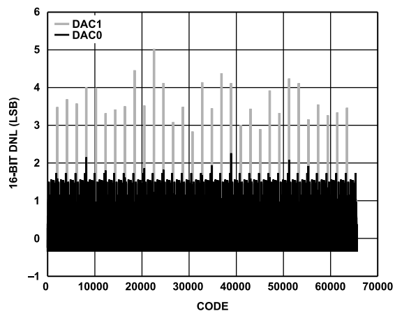
Figure 33. DNL, I_{OUTFS} = 26 mA, 16-Bit Resolution
