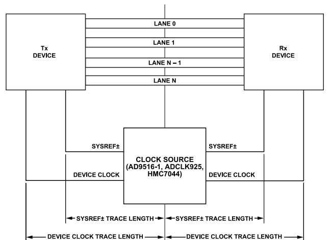
Figure 85. SYSREF \pm Signal and Device Clock Trace Length
