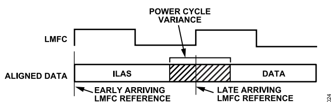
Figure 60. Link Delay &gt; LMFC Period Example
