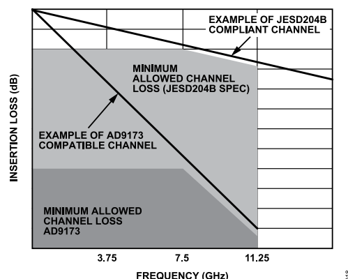
Figure 52. Insertion Loss Allowed
