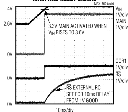
POWER-ON TIMING FOR 3.3V MAIN AND RESET SIGNAL
