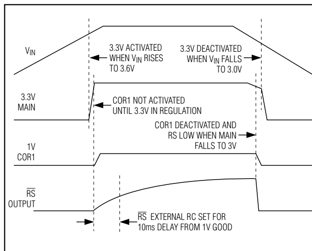
Figure 3. \overline{RS} and Power-On, Power-Off Timing for 3.3V and 1V Core
