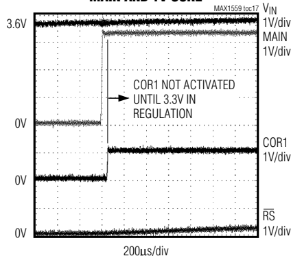
POWER-ON TIMING FOR 3.3V MAIN AND 1V CORE
