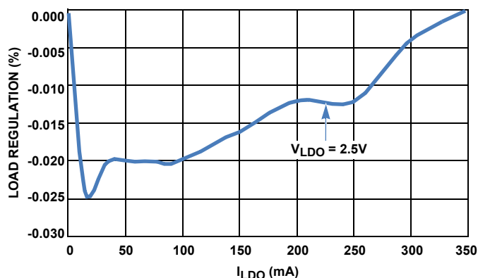
FIGURE 12. LDO LOAD REGULATION vs I_{LDO}
