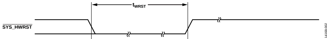
Figure 2. Reset Timing
