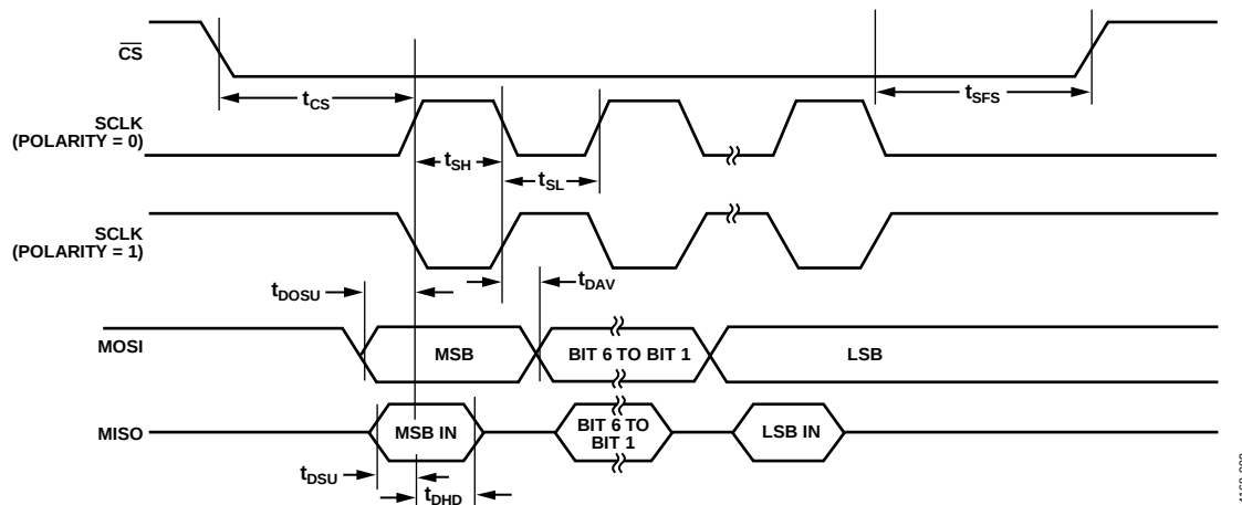
Figure 9. SPI Master Mode Timing (Phase = 0)
