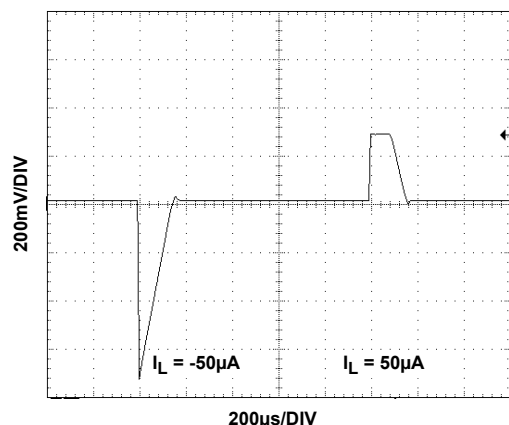
FIGURE 108. LOAD TRANSIENT RESPONSE
