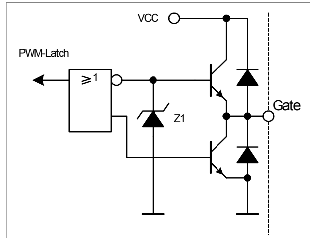
Figure 7 Gate Driver
