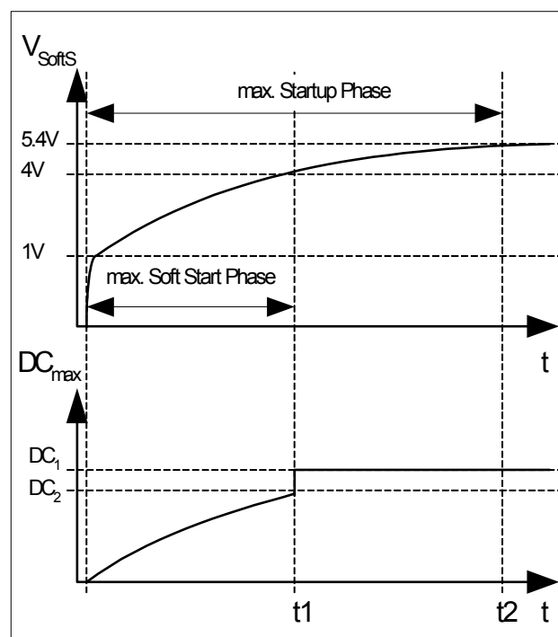
Figure 5 Startup Phase
