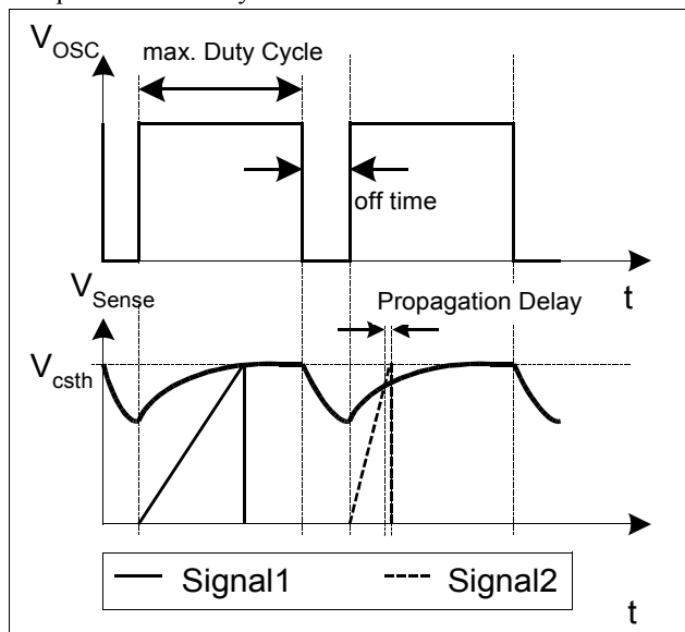
Figure 13 Dynamic Voltage Threshold V_{csth}
