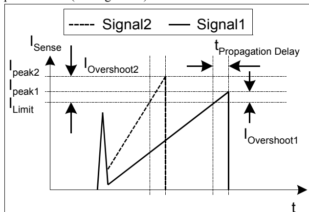
Figure 11 Current Limiting
