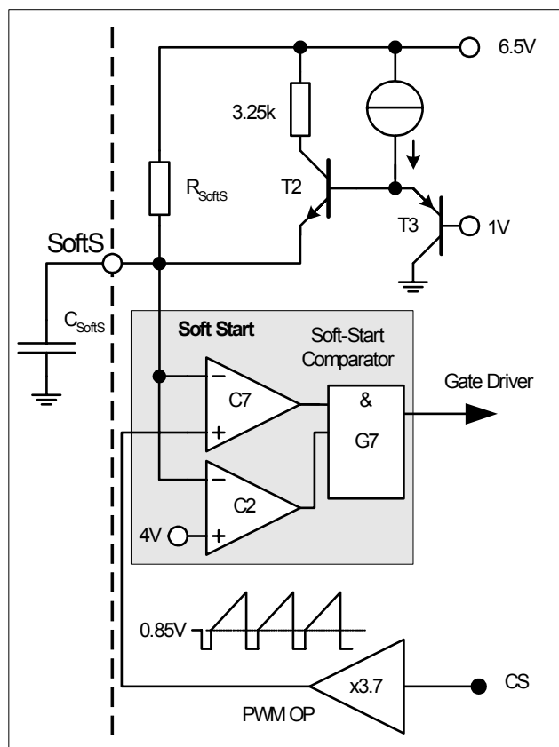
Figure 4 Soft Start
