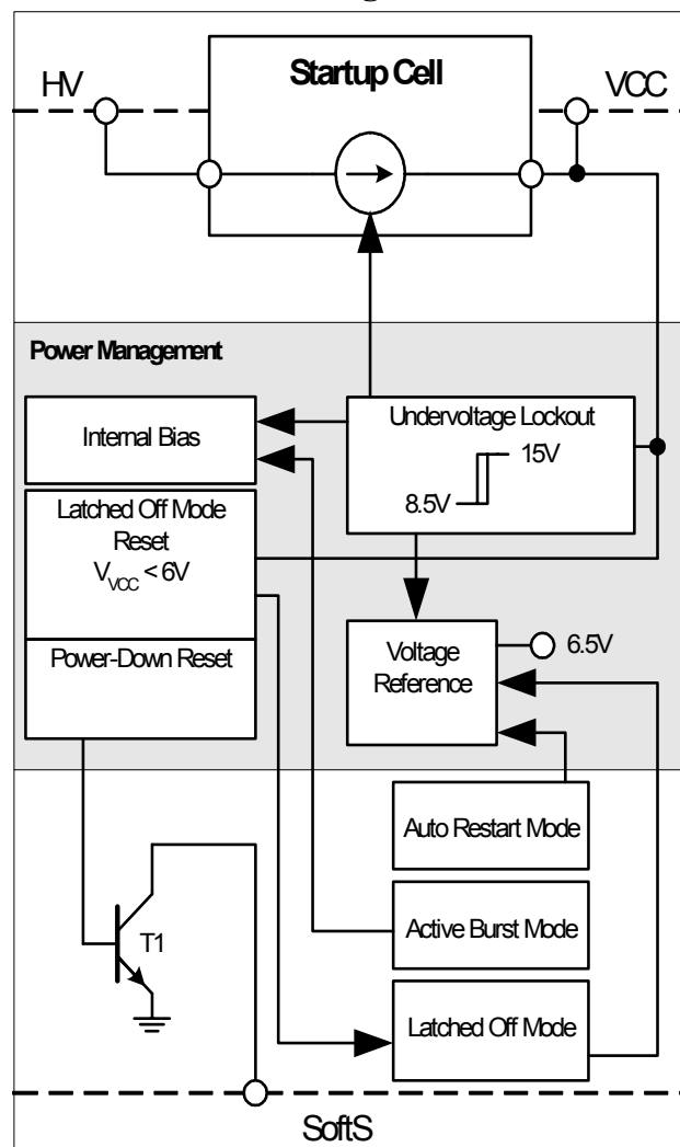
Figure 3 Power Management
