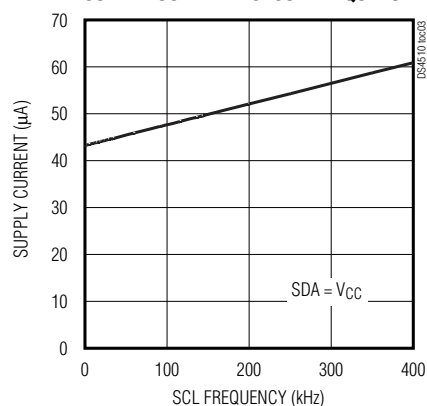
SUPPLY CURRENT vs. SCL FREQUENCY
