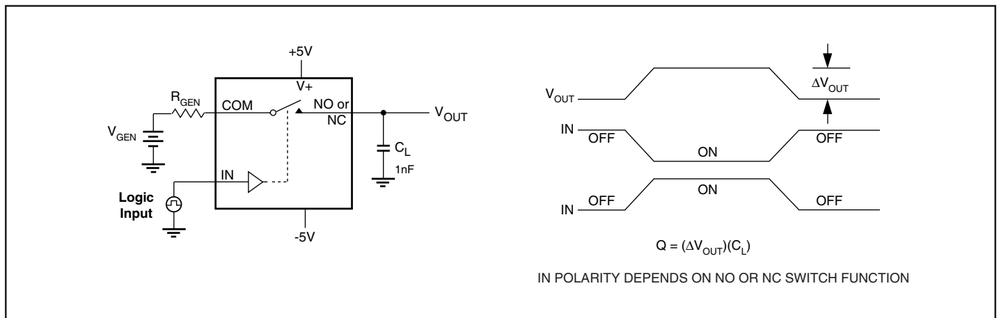
Figure 4. Charge Injection
