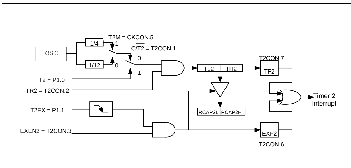
Figure 14. 16-Bit Capture Mode
