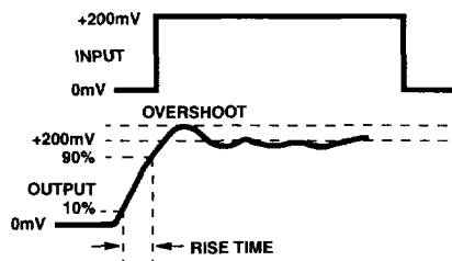
FIGURE 2. TRANSIENT RESPONSE
