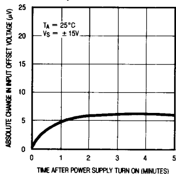
Warm-Up Drift
