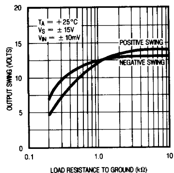
Output Voltage vs Load Resistance
