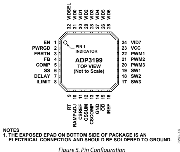
Figure 5. Pin Configuration
