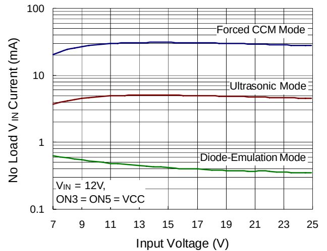
No Load V_{IN} Current vs. Input Voltage
