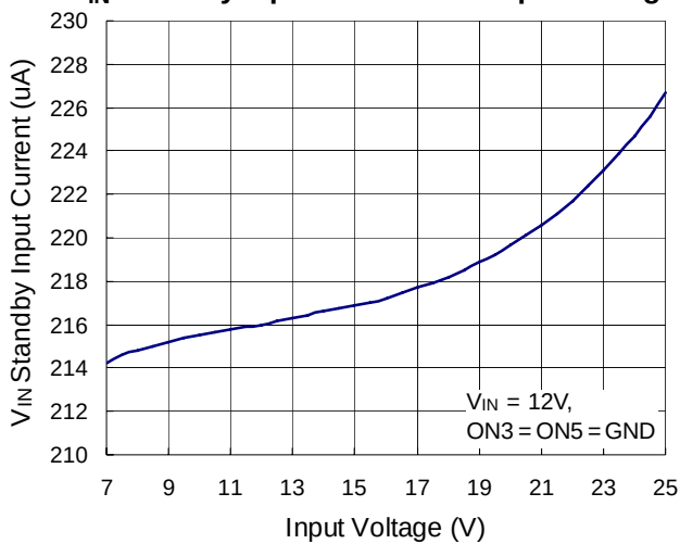
V_{IN} Standby Input Current vs. Input Voltage
