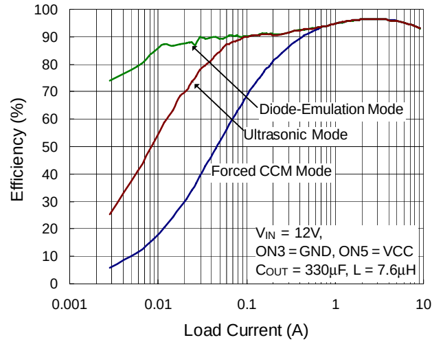
VOUT5 Efficiency vs. Load Current
