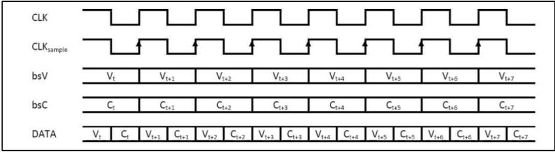
Figure 3: Timing diagram
