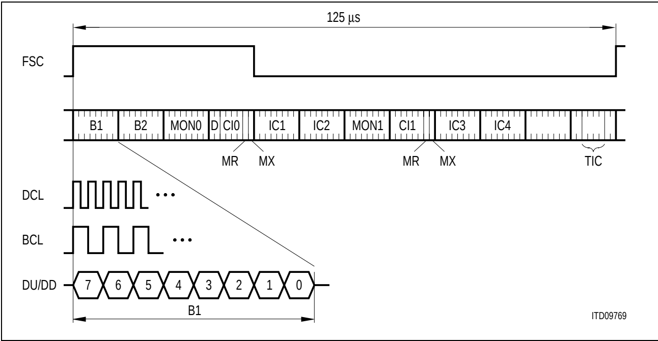
Figure 5 Example for IOM-2 Terminal Mode
