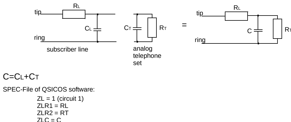
Figure 36 A simplified model of a subscriber line and an analog telephone set
