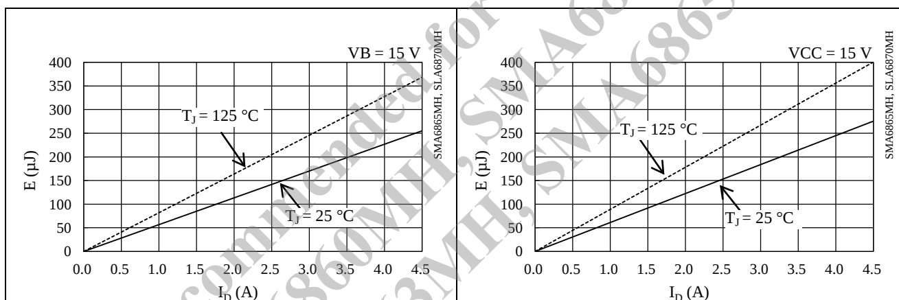
Figure 14-43. High-side Switching Loss
