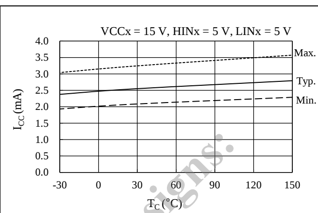
Figure 14-4. Logic Supply Current, I_{CC} vs. T_C ( HIN_x = 5\text{ V} , LIN_x = 5\text{ V} )
