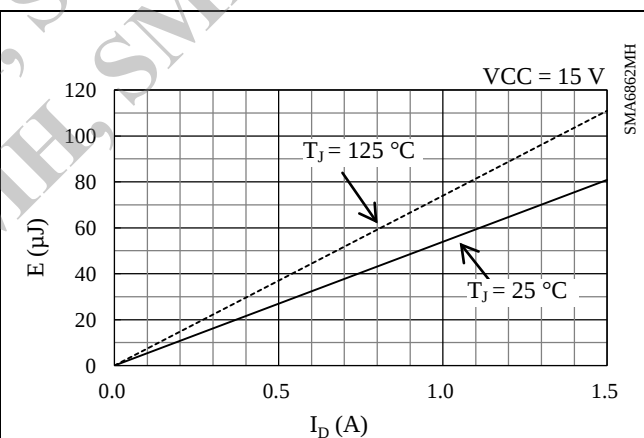
Figure 14-40. Low-side Switching Loss
