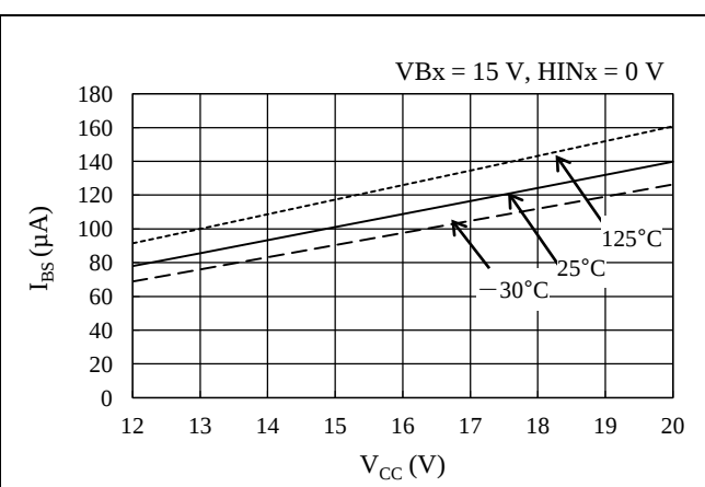
Figure 14-8. V_{Bx} Pin Voltage, V_B vs. Logic Supply Current, I_{BS} ( HIN_x = 0\text{ V} )
