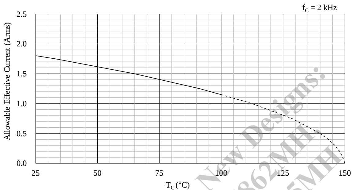
Figure 14-53. Allowable Effective Current ( f_C = 2 \text{ kHz} ): SLA6868MH
