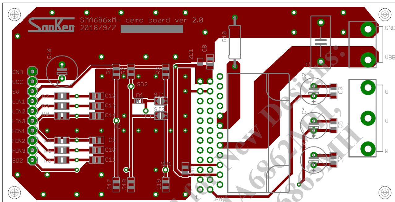
Figure 15-1. Top View
