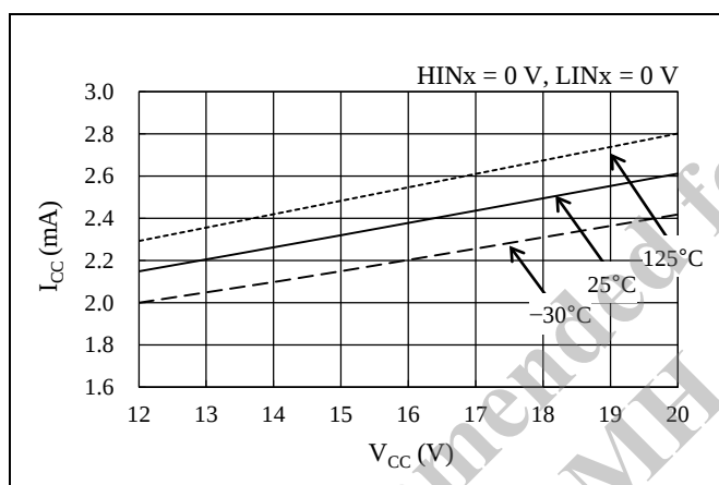
Figure 14-5. Logic Supply Current, I_{CC} vs. V_{CC} Pin Voltage, V_{CC}
