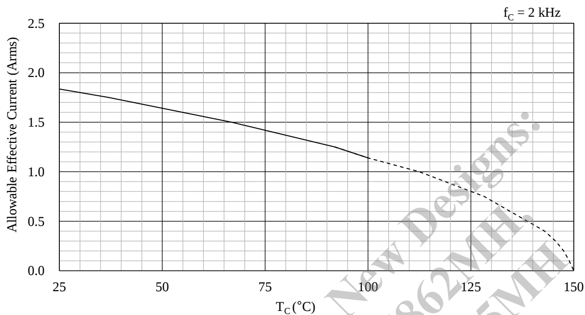
Figure 14-51. Allowable Effective Current ( f_C = 2 \text{ kHz} ): SMA6865MH
