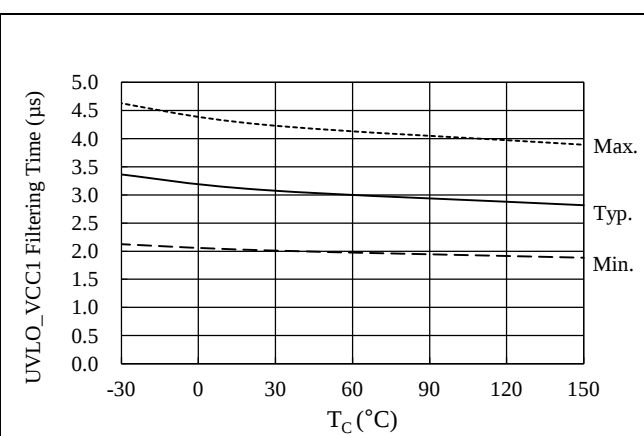
Figure 14-14. UVLO_VCC1 Filtering Time vs. T_C
