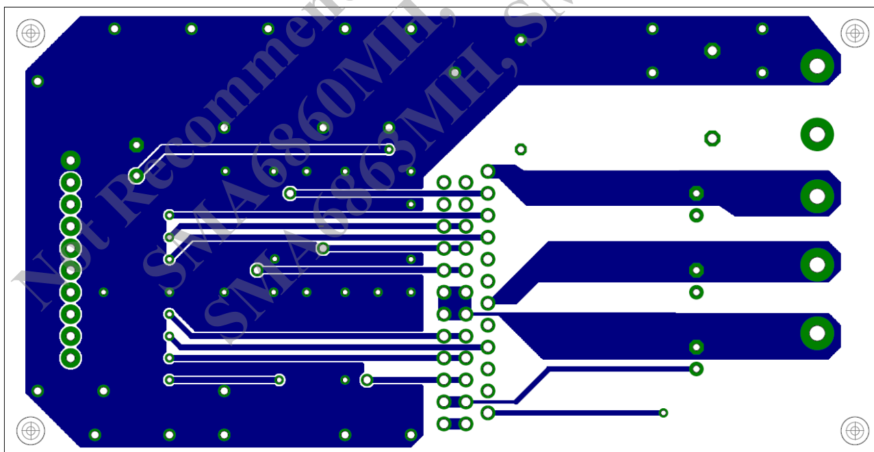
Figure 15-2. Bottom View
