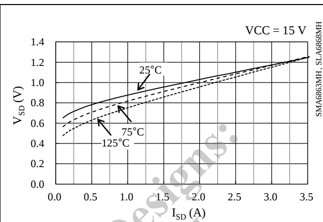
Figure 14-34. Power MOSFET V_{SD} vs. I_{SD}
