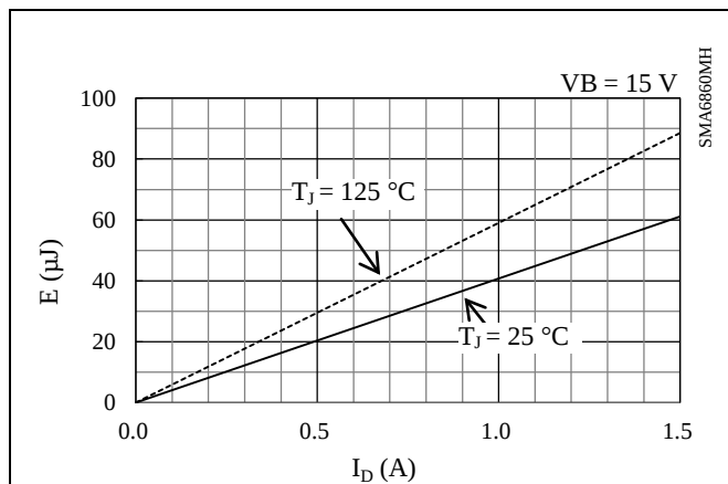
Figure 14-37. High-side Switching Loss
