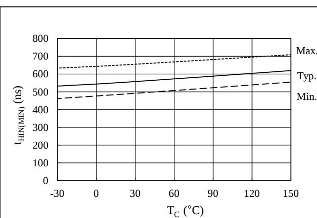
Figure 14-20. Low-side Turn-on Propagation Delay vs. T_C (from LINx to LOx)
