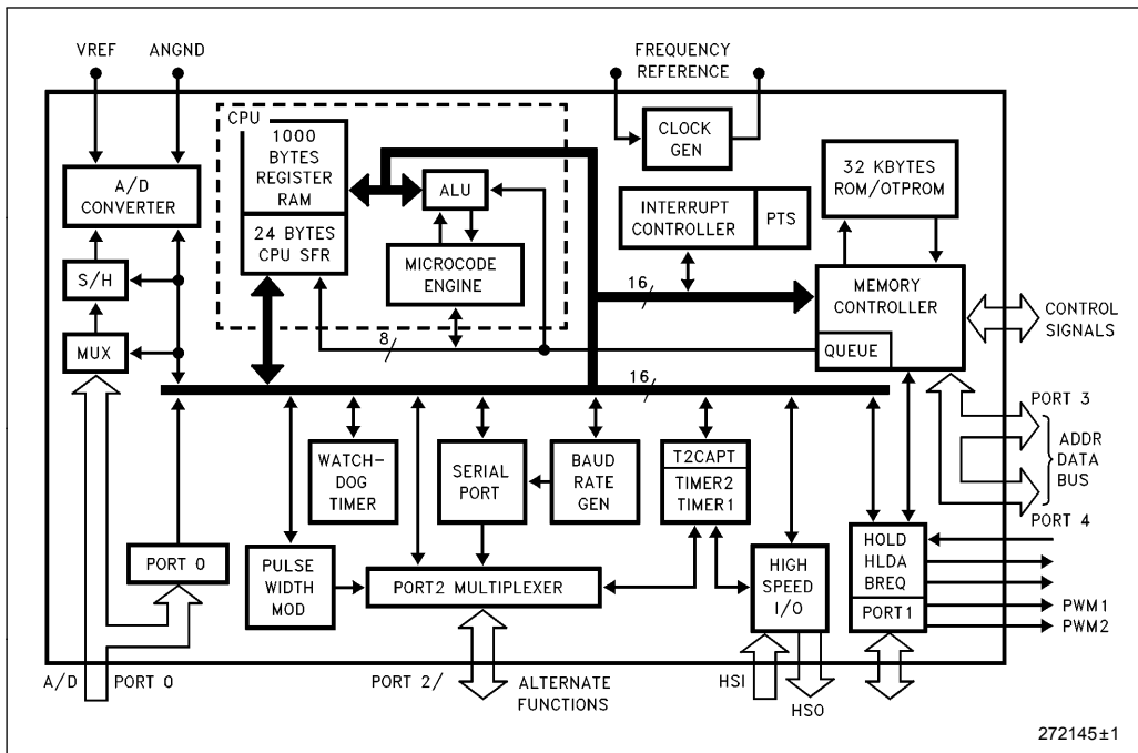
Figure 1.8XC196KD Block Diagram
