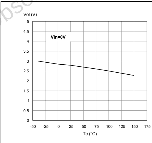
Figure 23. Open-load off-state detection threshold
