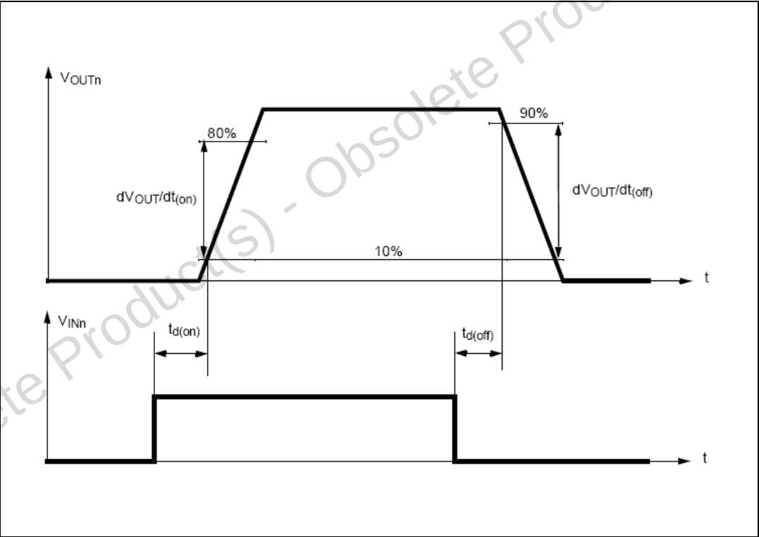
Figure 5. Switching characteristics
