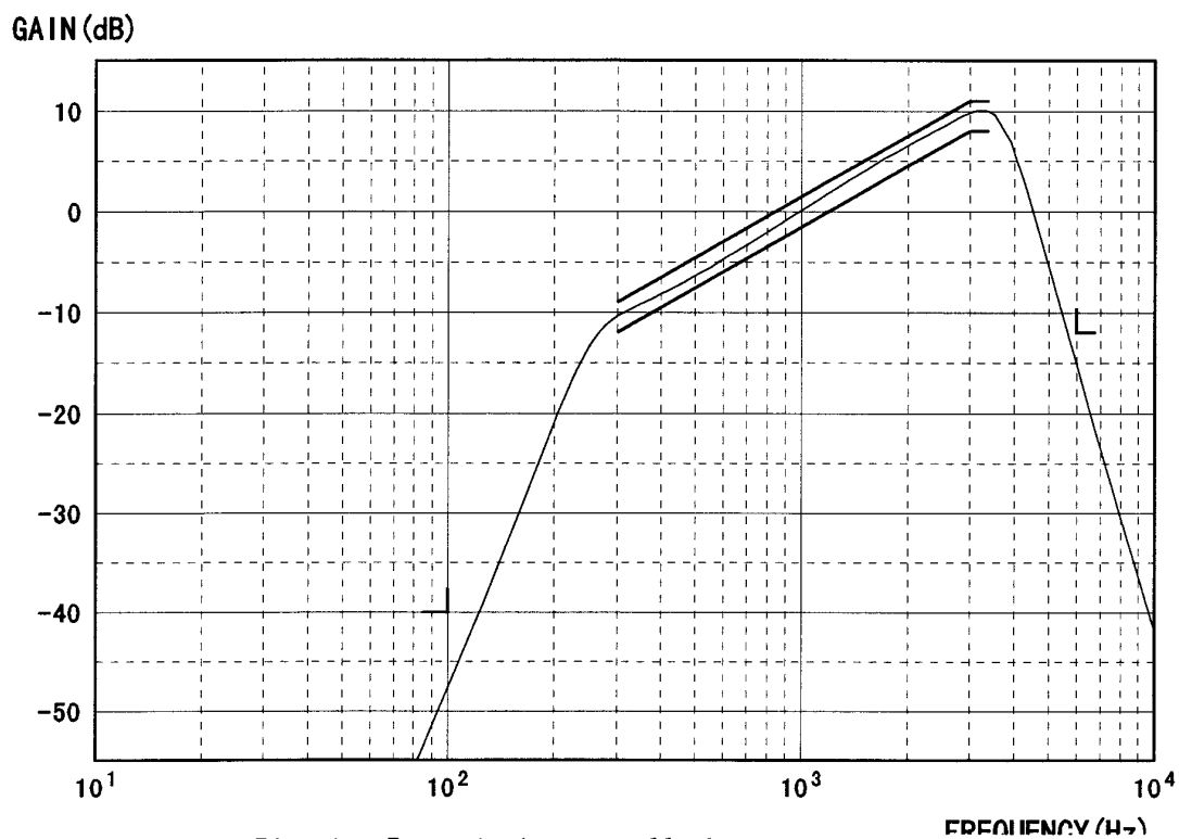
Fig. 1 Transmission overall characteristics
