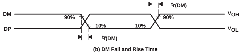
Figure 5-2. USB Data Signal Rise and Fall Times
