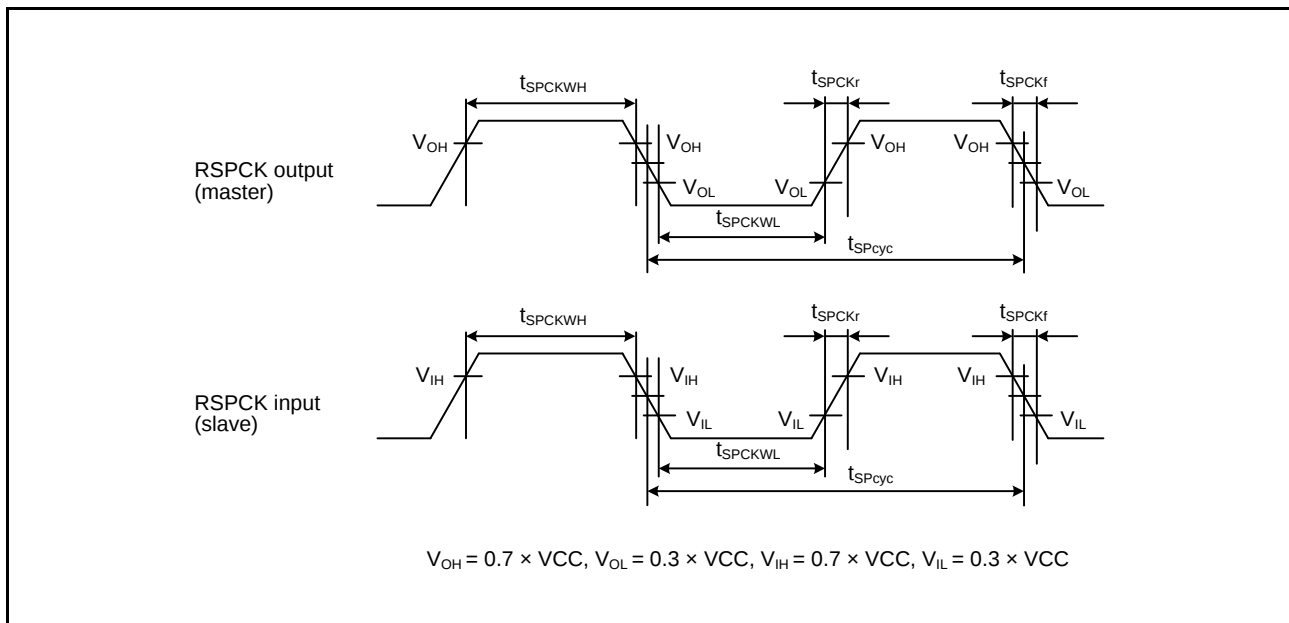
Figure 2.68 RSPI Clock Timing
