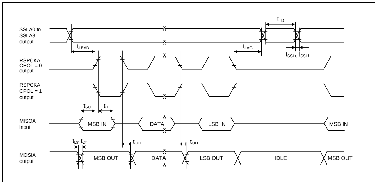
Figure 2.69 RSPI Timing (Master, CPHA = 0) (Bit Rate: PCLKA Division Ratio Set to a Value Other Than 1/2)
