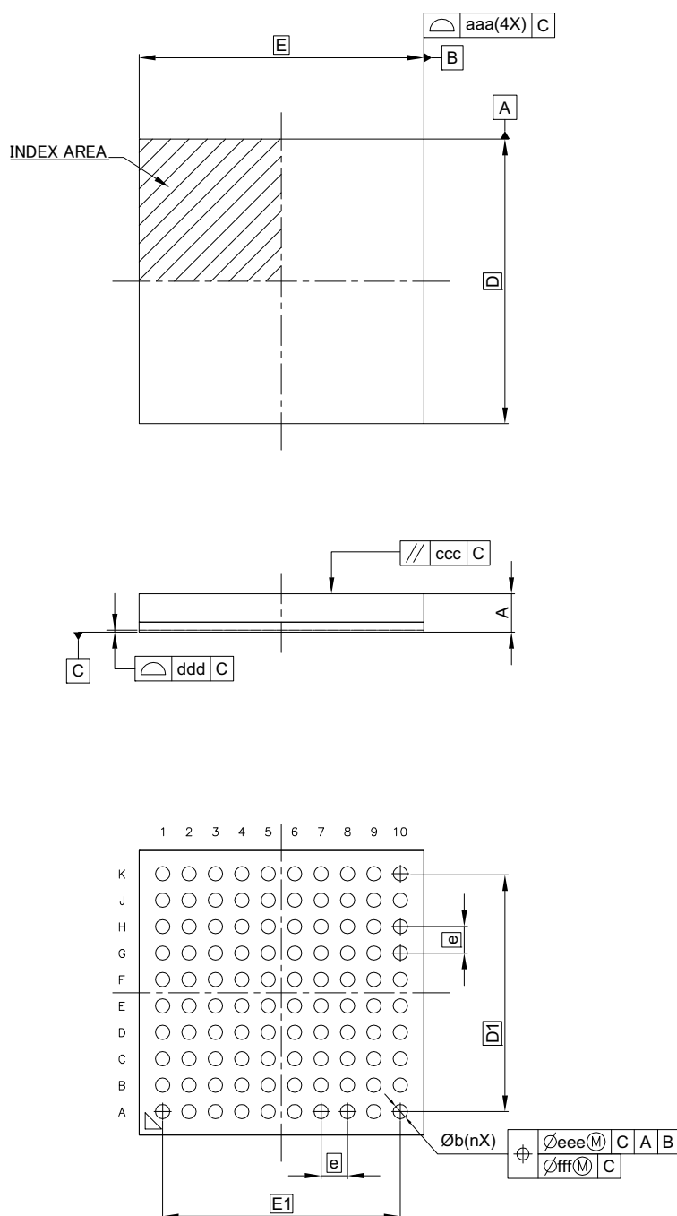
Figure D 100-Pin TFLGA (PTLG0100JB-A)
