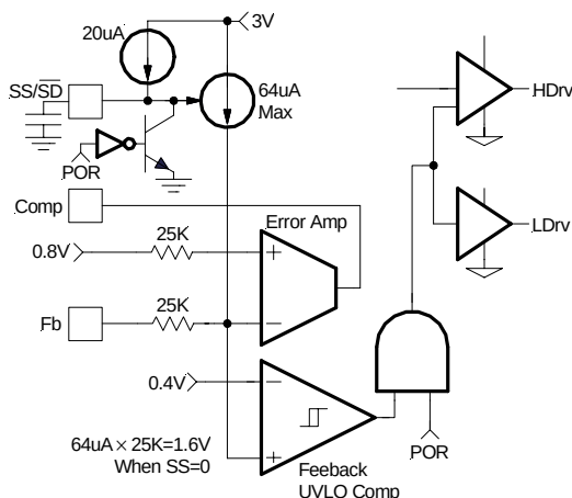
Figure 3 - Soft-start circuit for IRU3137.
