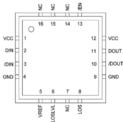
16-Pin QFN
