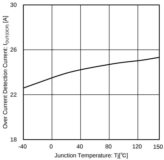
Figure 25. Over Current Detection Current vs Junction Temperature
