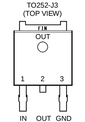
Figure 2. Pin Configuration
