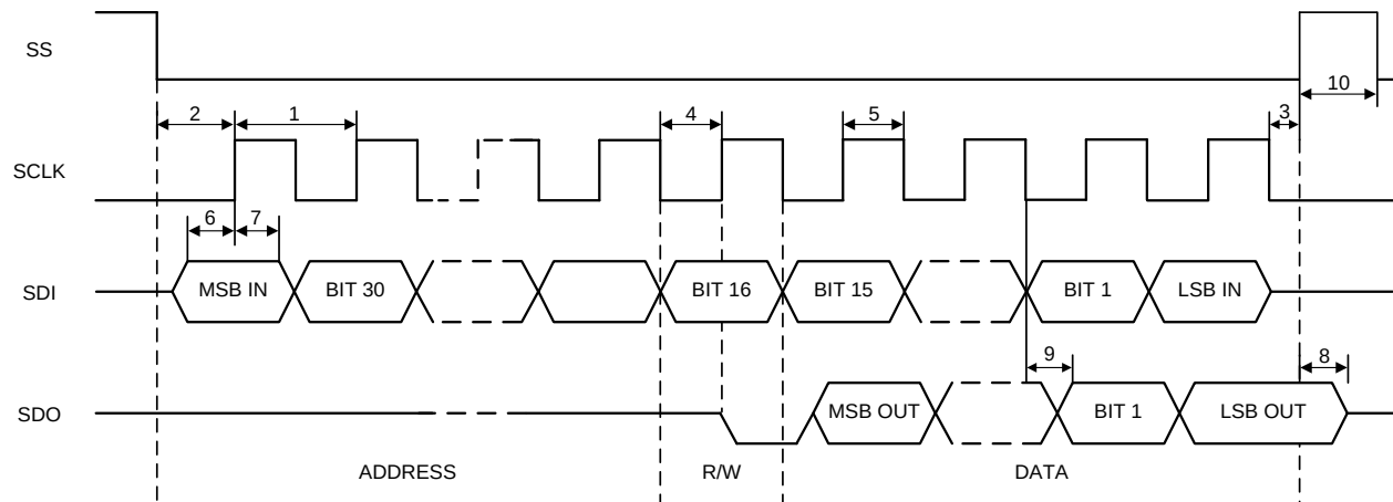
Figure 2. SPI Timing
