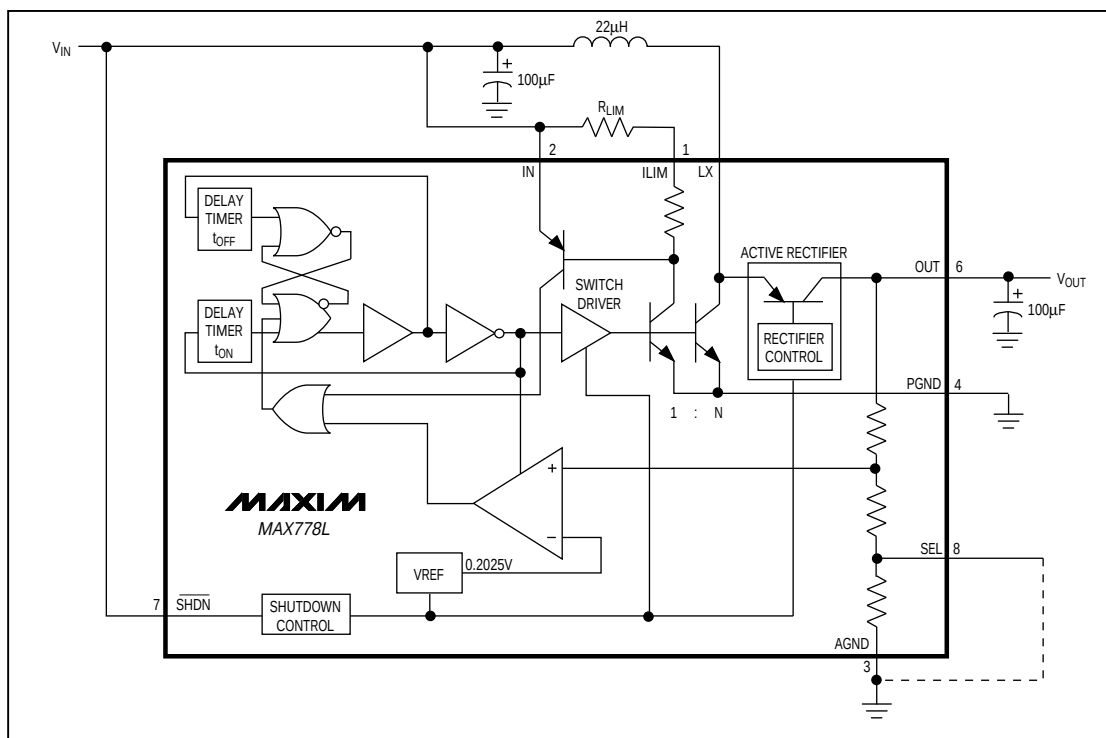
Figure 1. MAX7778L Block Diagram
