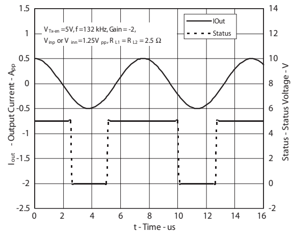
Figure 10. Output load detection.
