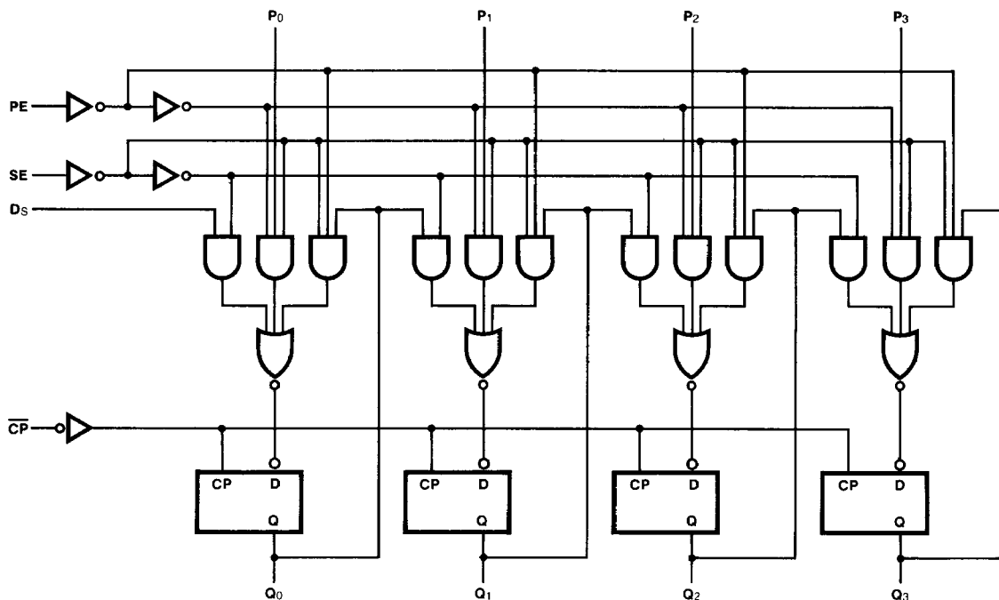
LOGIC DIAGRAM
