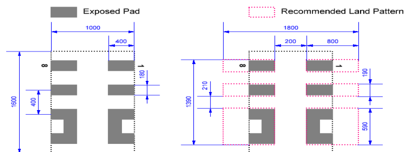
Figure 2. SLG59M1598V Package Dimensions and Recommended Land Pattern
