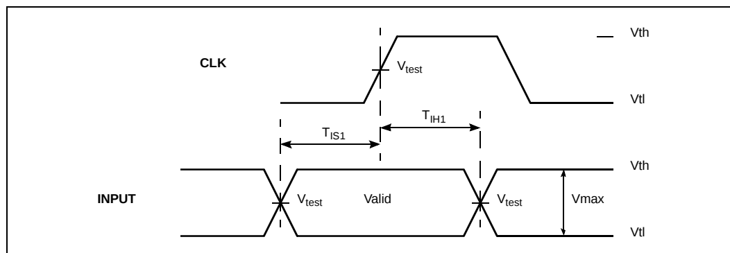
Figure 12. Input Timing Measurement Waveforms
