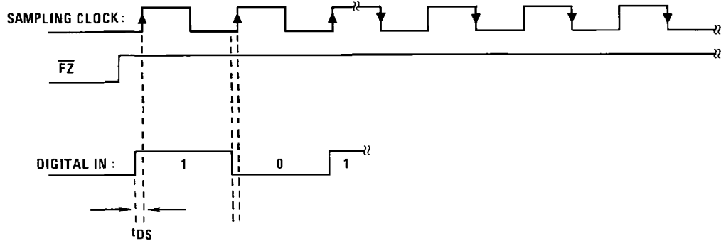
FIGURE 2 – CVSD TIMING DIAGRAM
