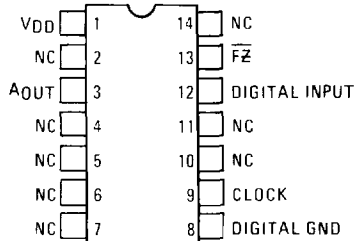
HC-55536 (CERAMIC DIP) TOP VIEW
