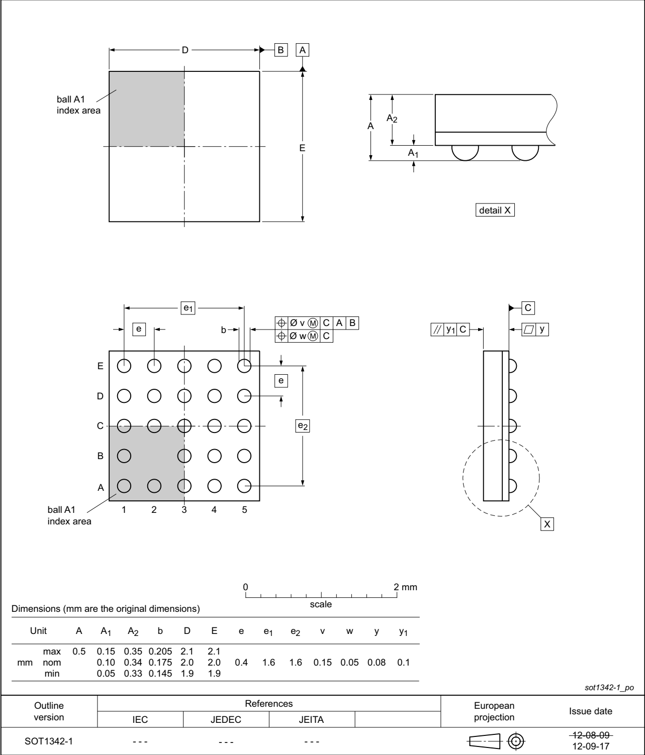
Fig 41. Package outline SOT1342-1 (XFBGA24); EX option
