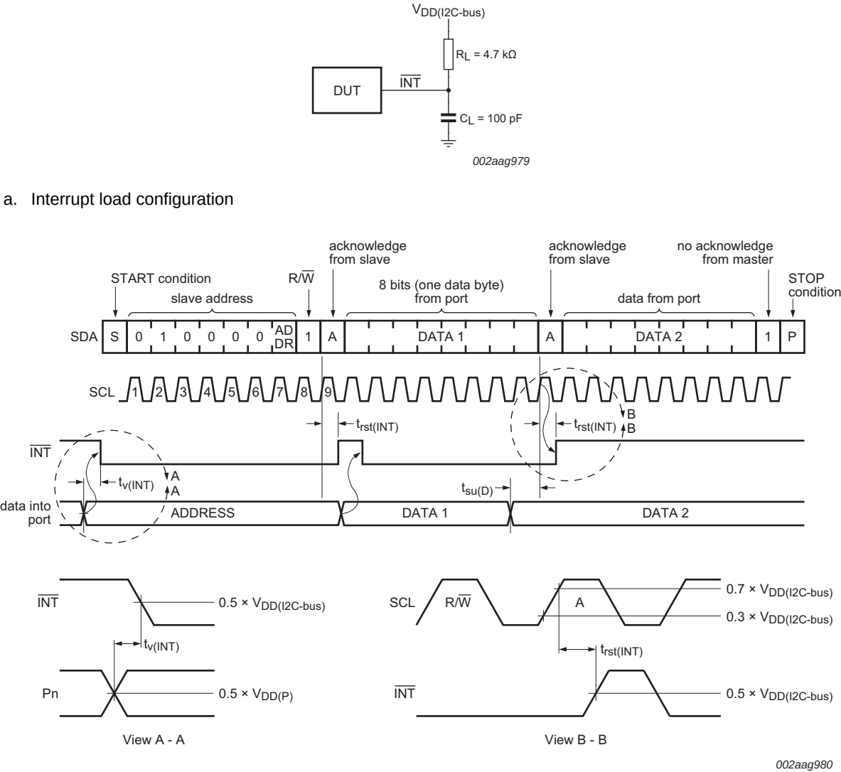
b. Voltage waveforms C L includes probe and jig capacitance. All inputs are supplied by generators having the following characteristics: PRR ≤ 10 MHz; Z 0 = 50 Ω; t r /t f ≤ 30 ns. All parameters and waveforms are not applicable to all devices.
