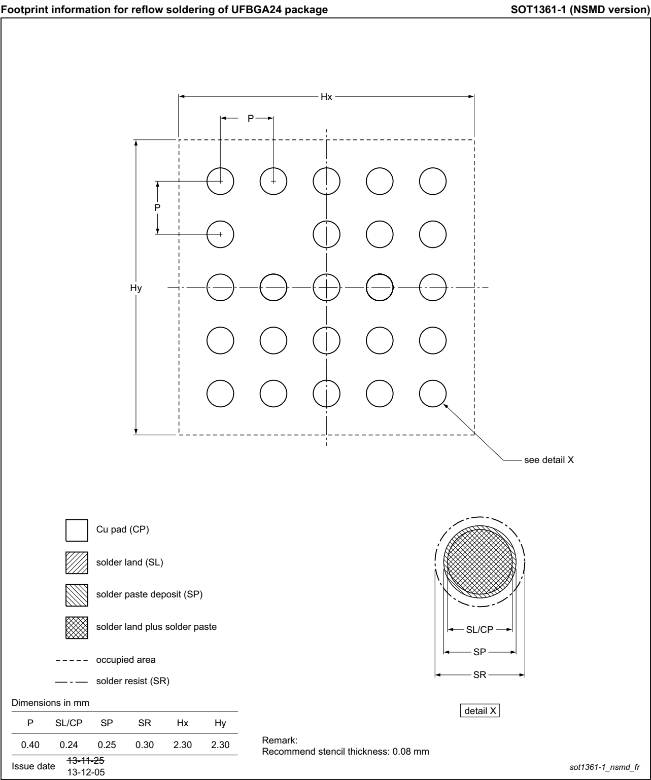
Fig 52. PCB footprint for SOT1361-1 (UFBGA24, Non-Solder Mask Defined version), ER option; reflow soldering
