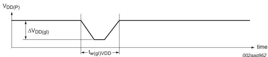
Fig 24. Glitch width and glitch height
