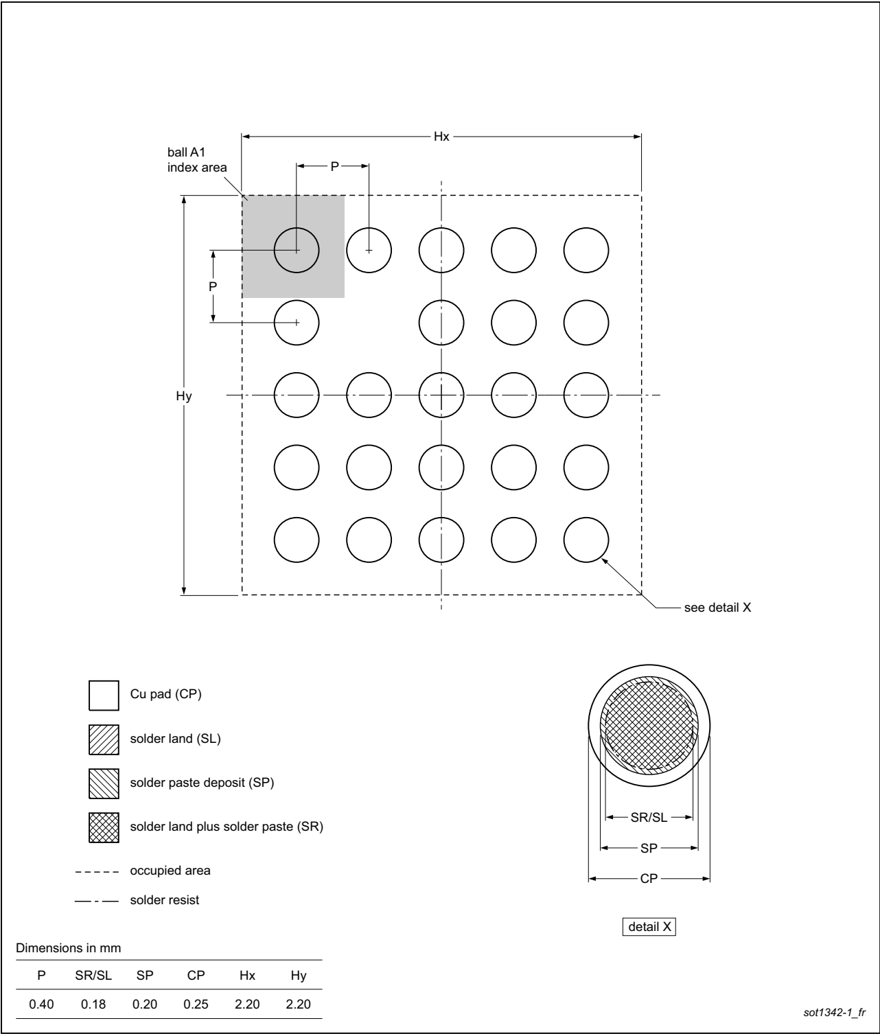
Footprint information for reflow soldering of XFBGA24 package
