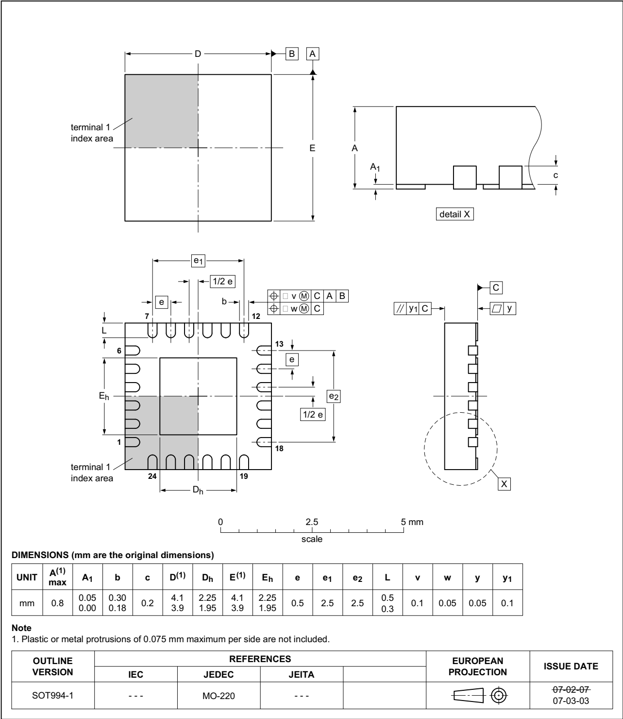
Fig 38. Package outline SOT994-1 (HWQFN24)
