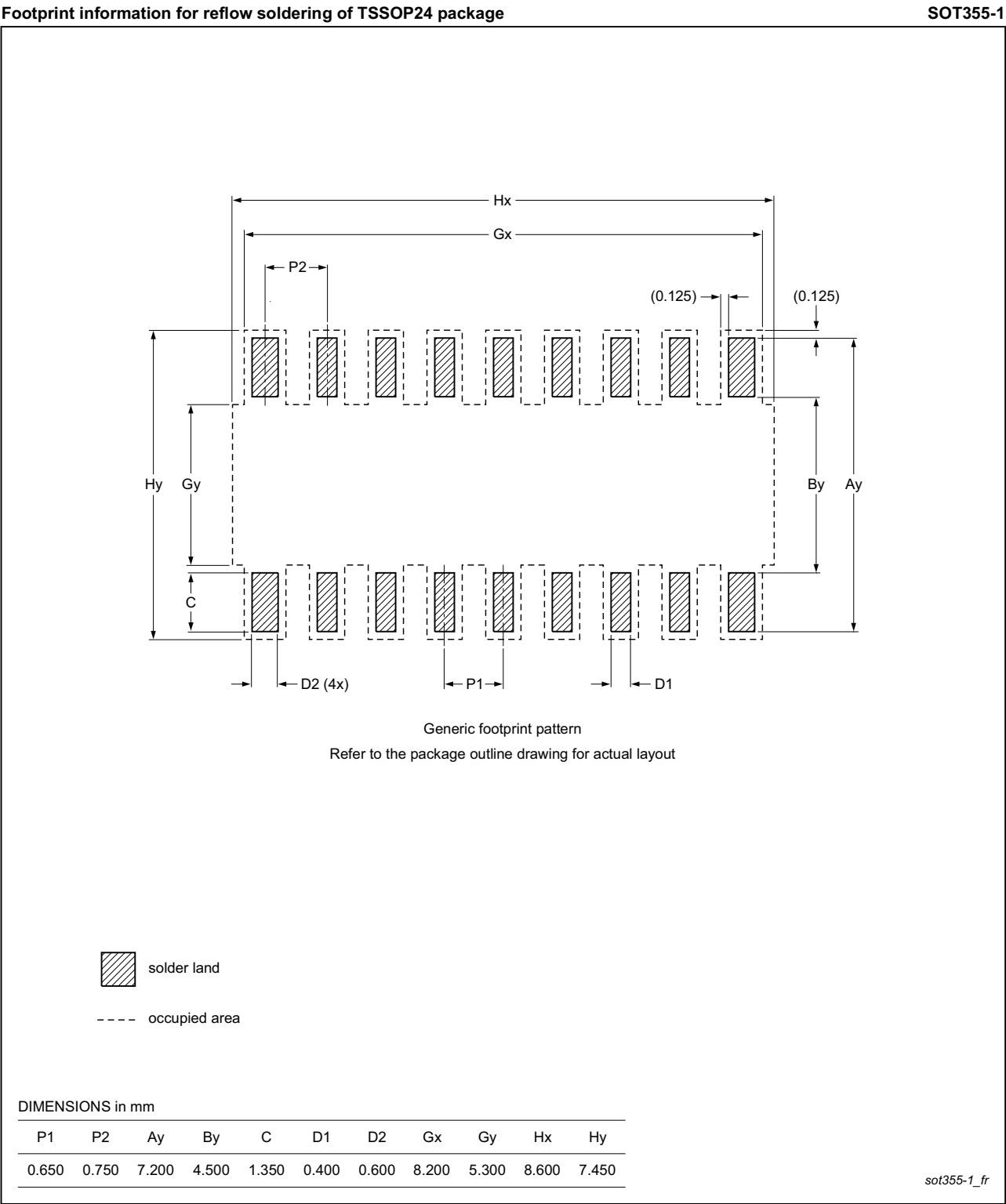
Fig 46. PCB footprint for SOT355-1 (TSSOP24); reflow soldering
