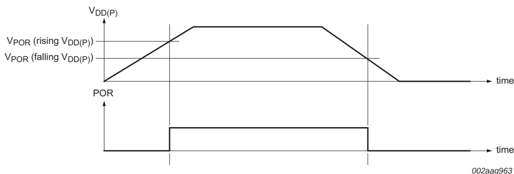
Fig 25. Power-on reset voltage ( V_{POR} )
