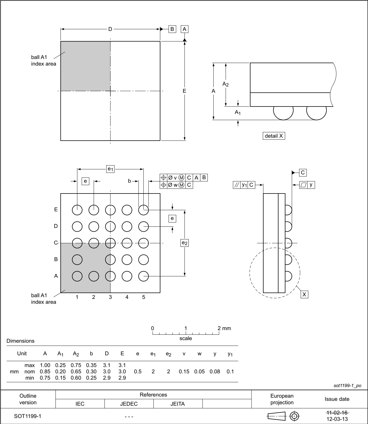
Fig 40. Package outline SOT1199-1 (VFBGA24)
