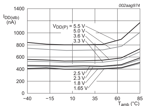
Fig 27. Standby supply current versus ambient temperature
