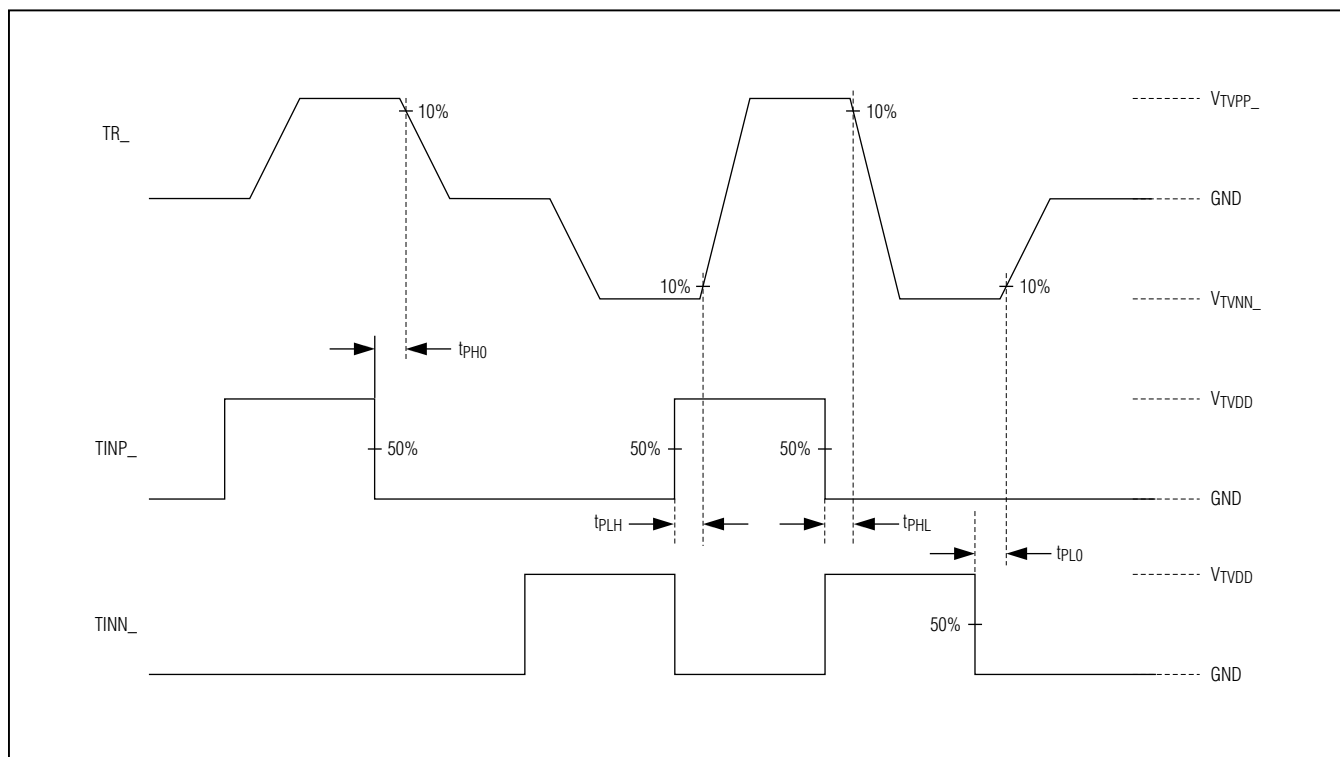
Figure 3. Propagation Delay Timing
