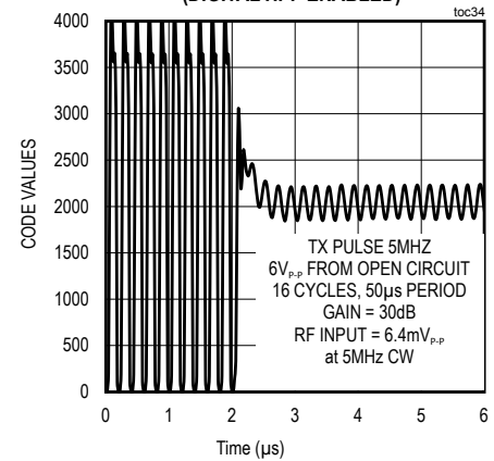
VGA OVERLOAD RECOVERY (DIGITAL HPF ENABLED)
