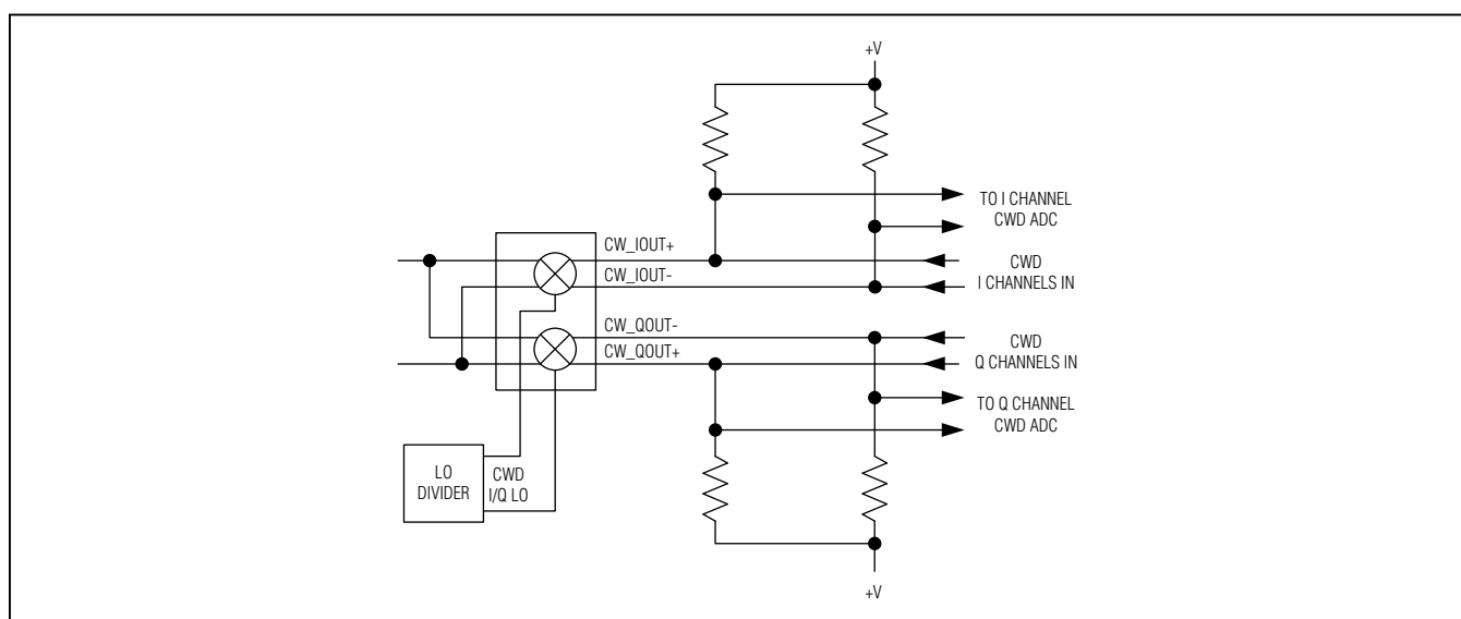
Figure 10. CWD Output Beamforming Example
