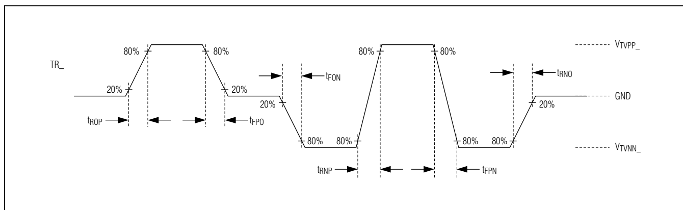
Figure 4. Output Rise/Fall Timing
