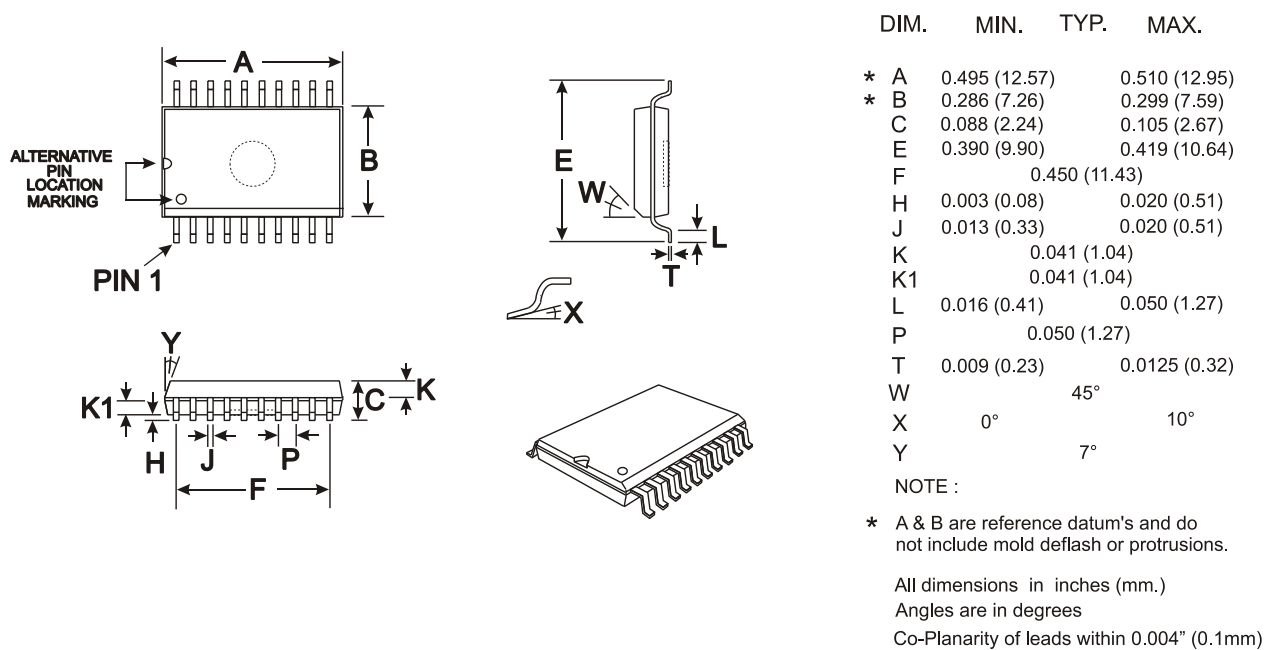
Figure 17 20-Lead SOIC Mechanical Outline: Order as part no. CMX649D3
